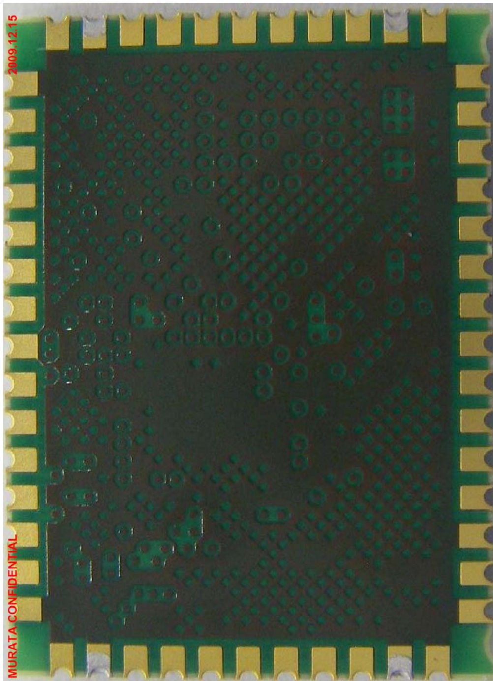
Bluetooth Module BottomView without shield
