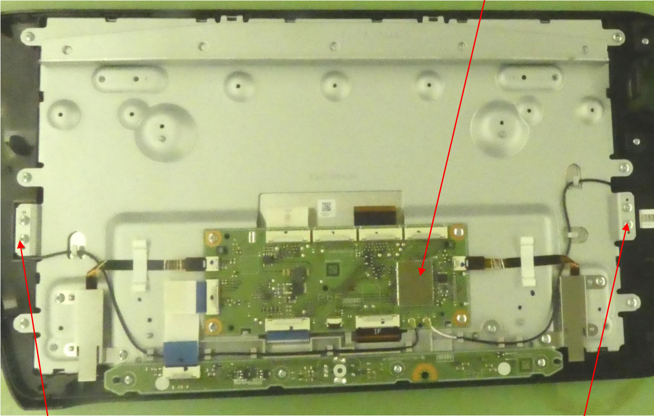
Panel plate Inside view
