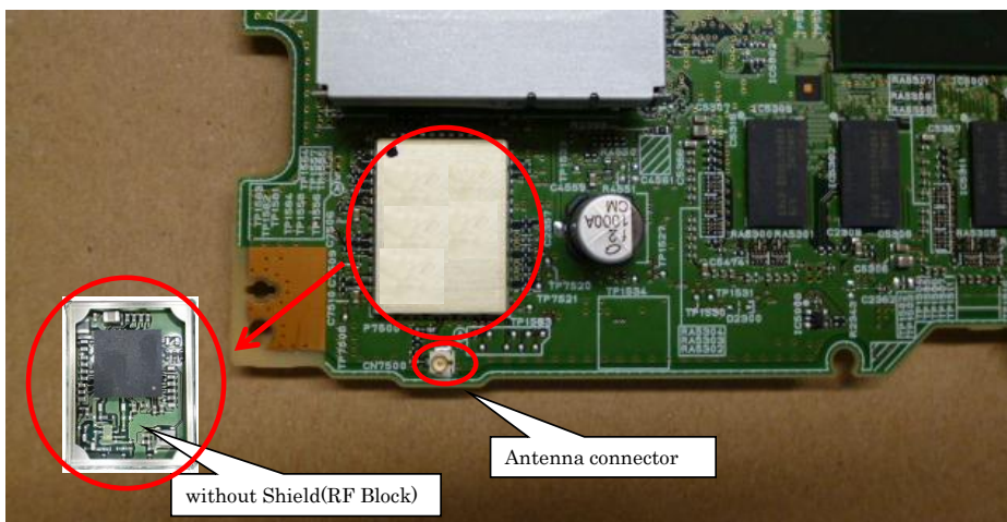
Fig.6 RF Block
