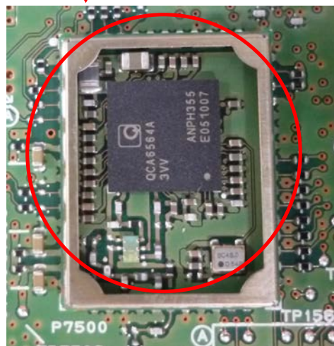
Fig.8 RF Block Detail(Without Shield)
