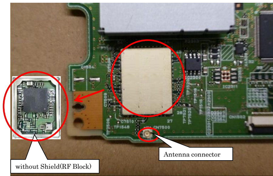
Fig.5 RF Block
