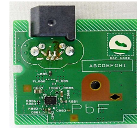
[KEY PCB / Solder Side]
