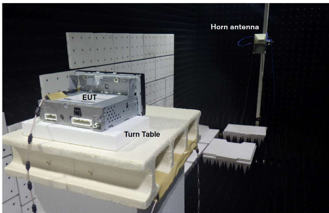
Test Setup
