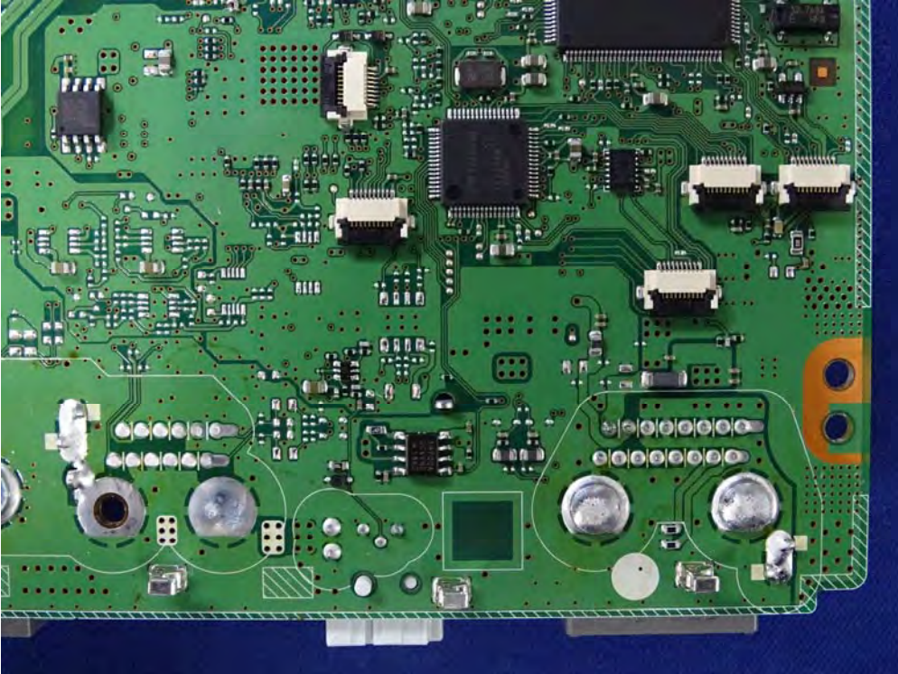
(73) EUT Photo
