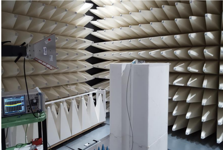
Figure F5. DUT Setup - Radiated
