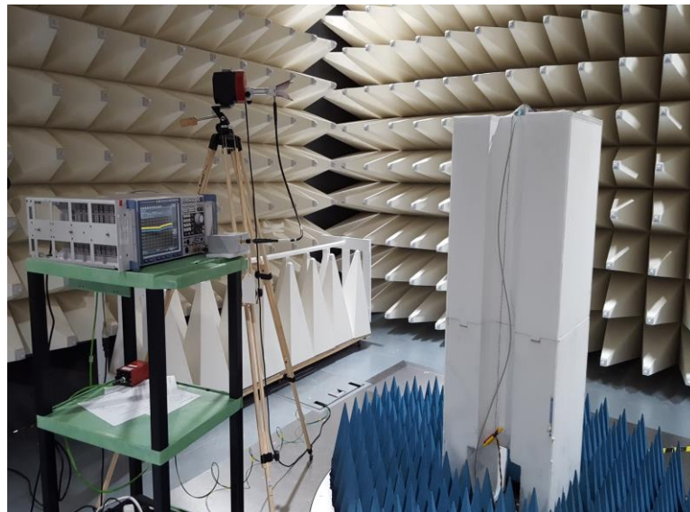
Figure F4. Radiated Setup – High Range
