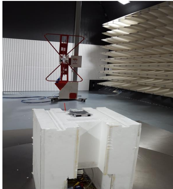
Figure F6. DUT Setup - Radiated
