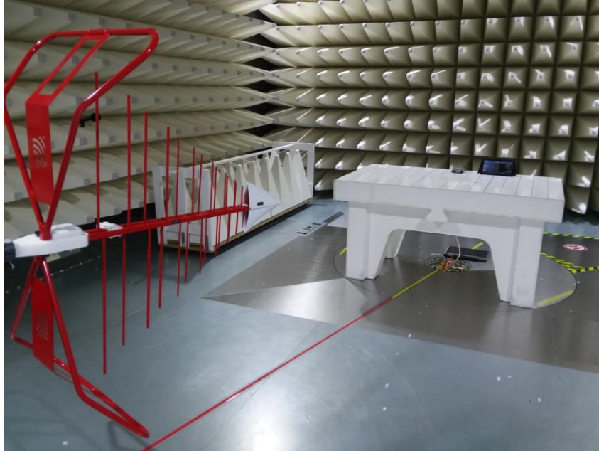
Figure B6. Radiated Setup – Low Range
