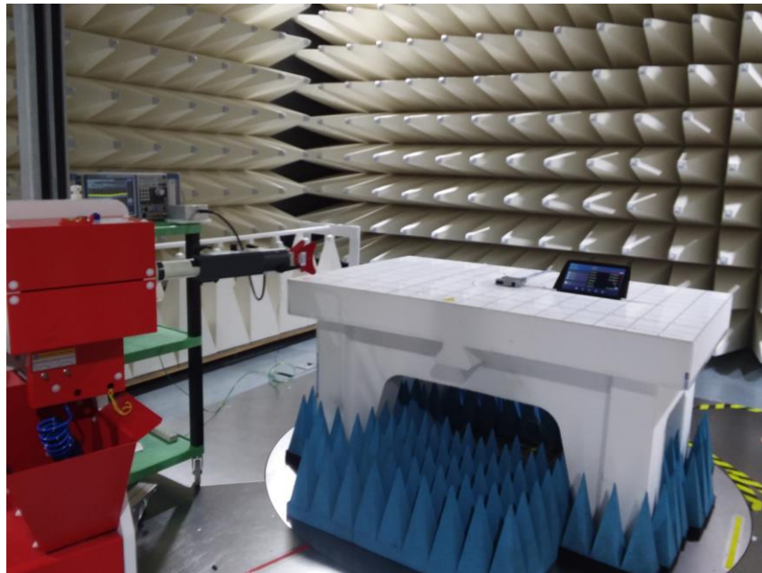
Figure B7. Radiated Setup – High Range
