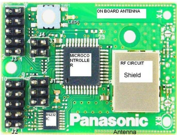
PAN802154 TOP VIEW WITH ALL OPTIONS INCLUDED: LED, TOUCH SWITCH, J1, J2, J3, J4, RS232 IC
