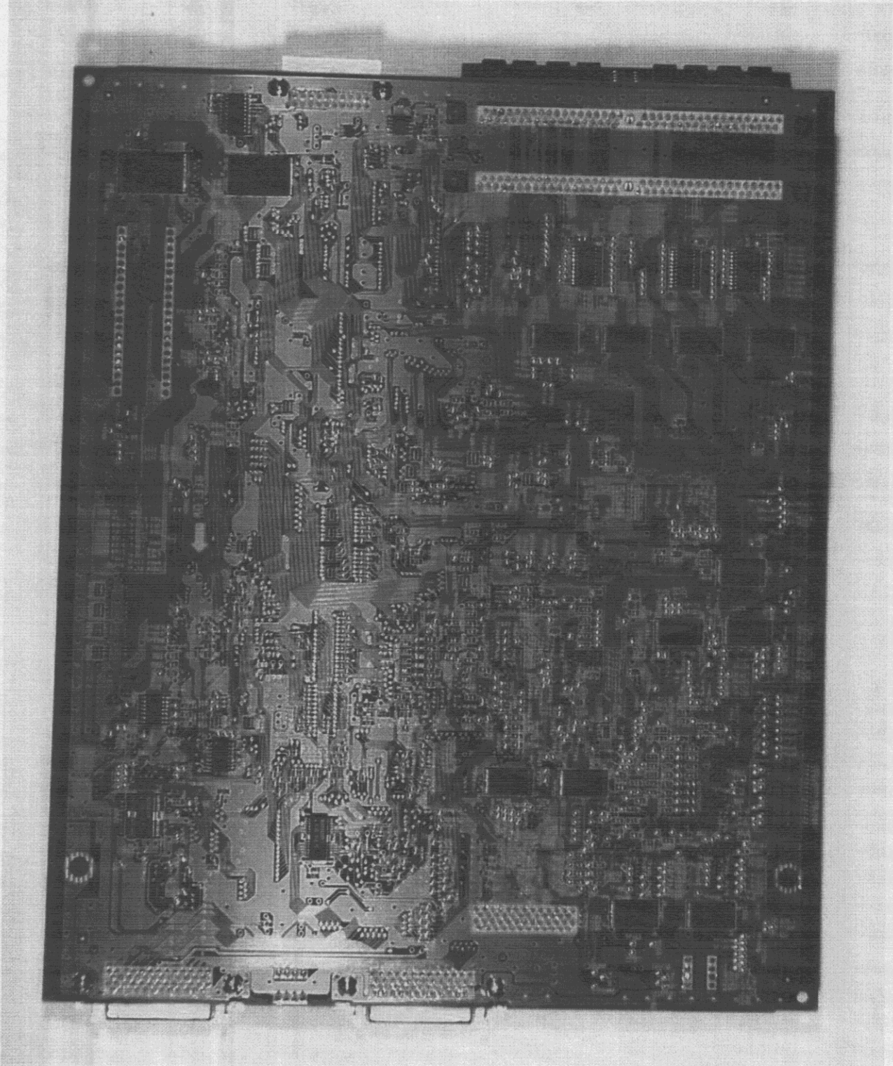
Photo 16 Bottom view of Duplicator Board.
