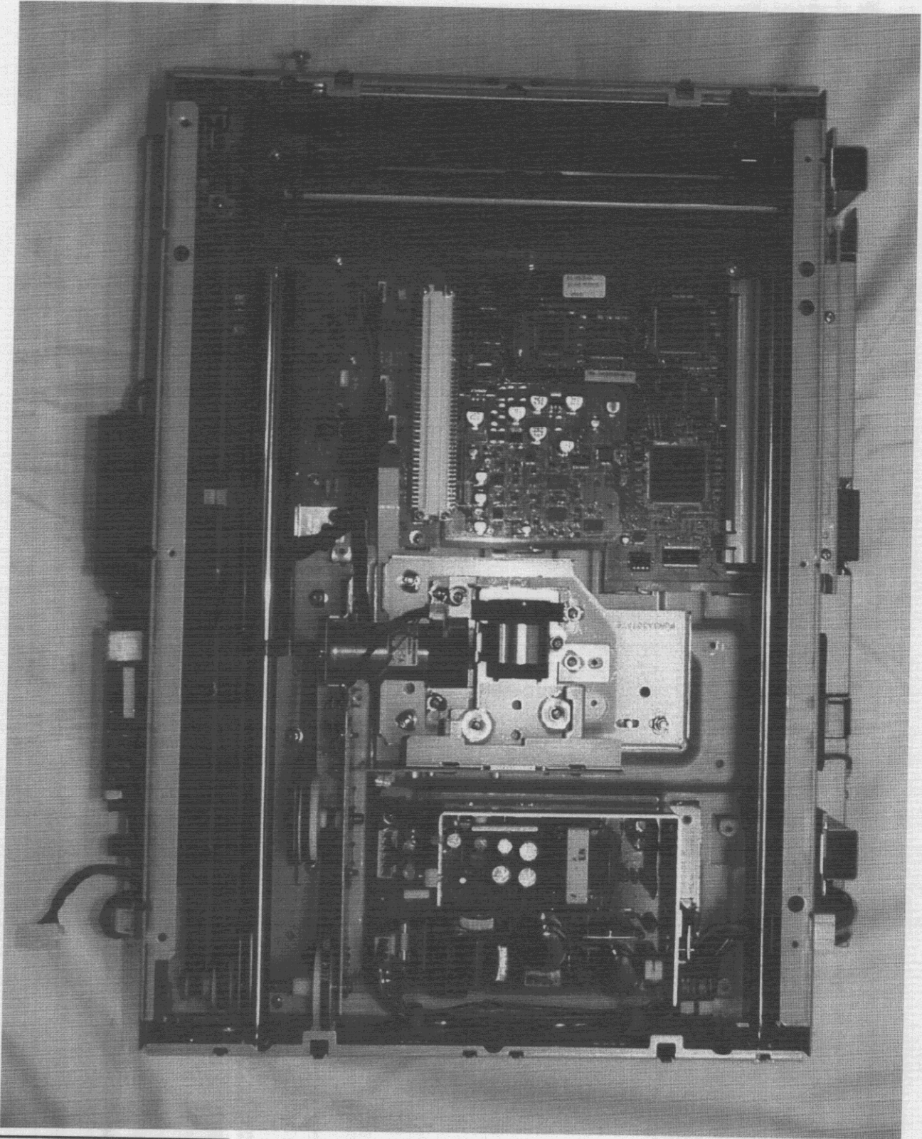
Photo 4 Top side view without Upper plate, Blind plate A and B.
