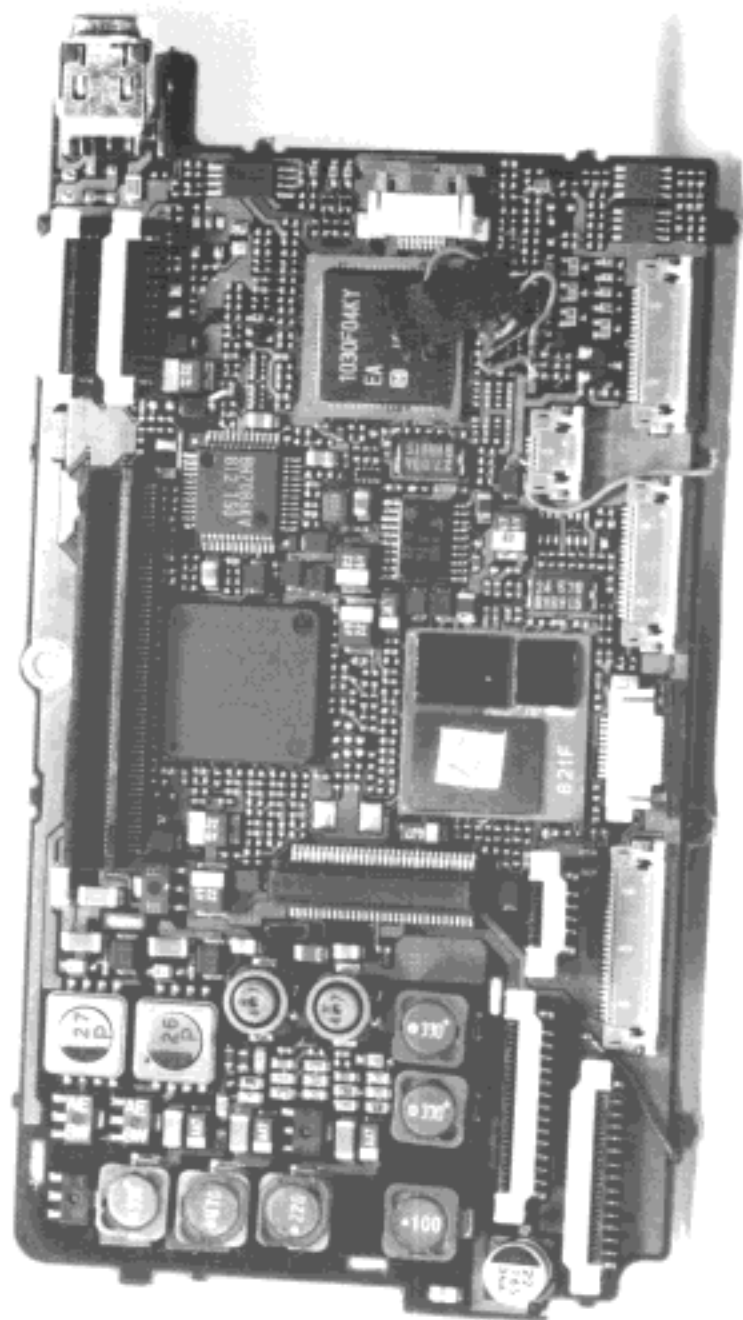
Main PCB (TOP VIEW)
