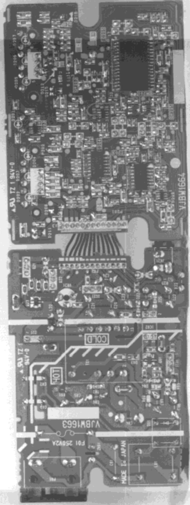
AC Adaptor PCB (BOTTOM VIEW)
