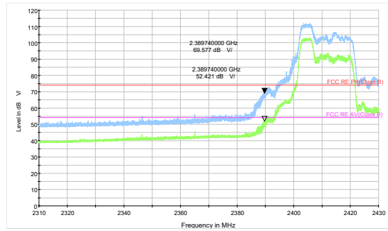
802.11ax HE20 52-Tone-CH1 Peak+ Average
