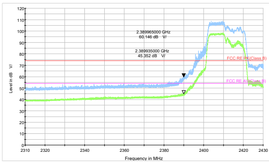
802.11ax HE20 106-Tone-CH1 Peak+ Average
