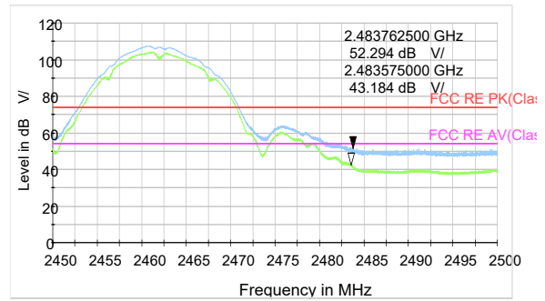
802.11b-Channel 11 Peak+ Average
