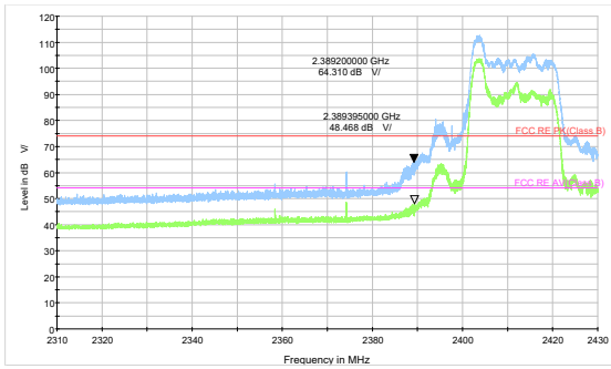
802.11ax HE20 26-Tone-CH1 Peak+ Average
