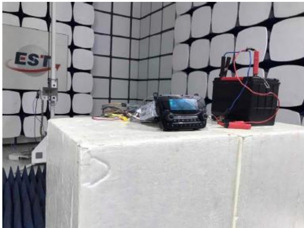
Above 1GHz
