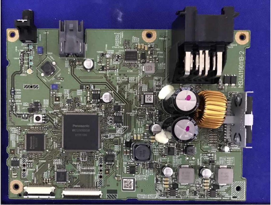
MAIN BOARD_B SIDE
