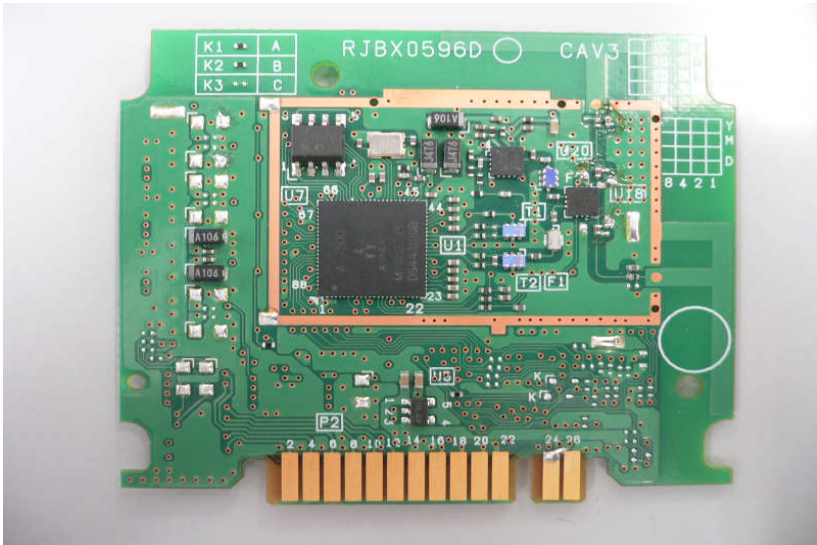
the reverse side (without SHIELD PLATE)
