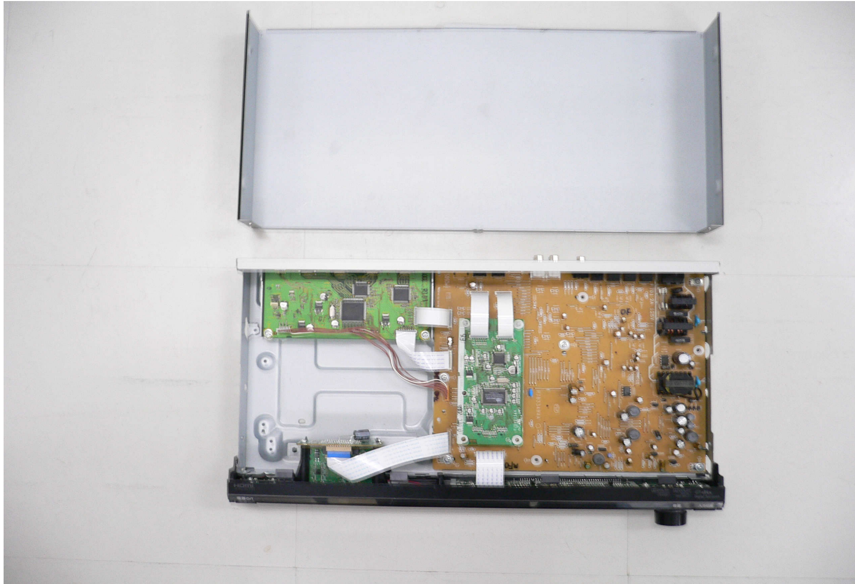
Internal picture [SU-ZT1]
