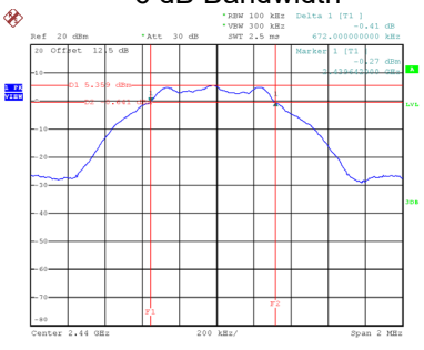
6 dB Bandwidth
