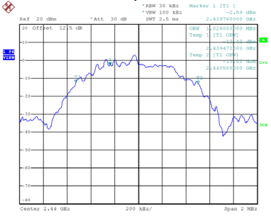
99 % Occupied Bandwidth
