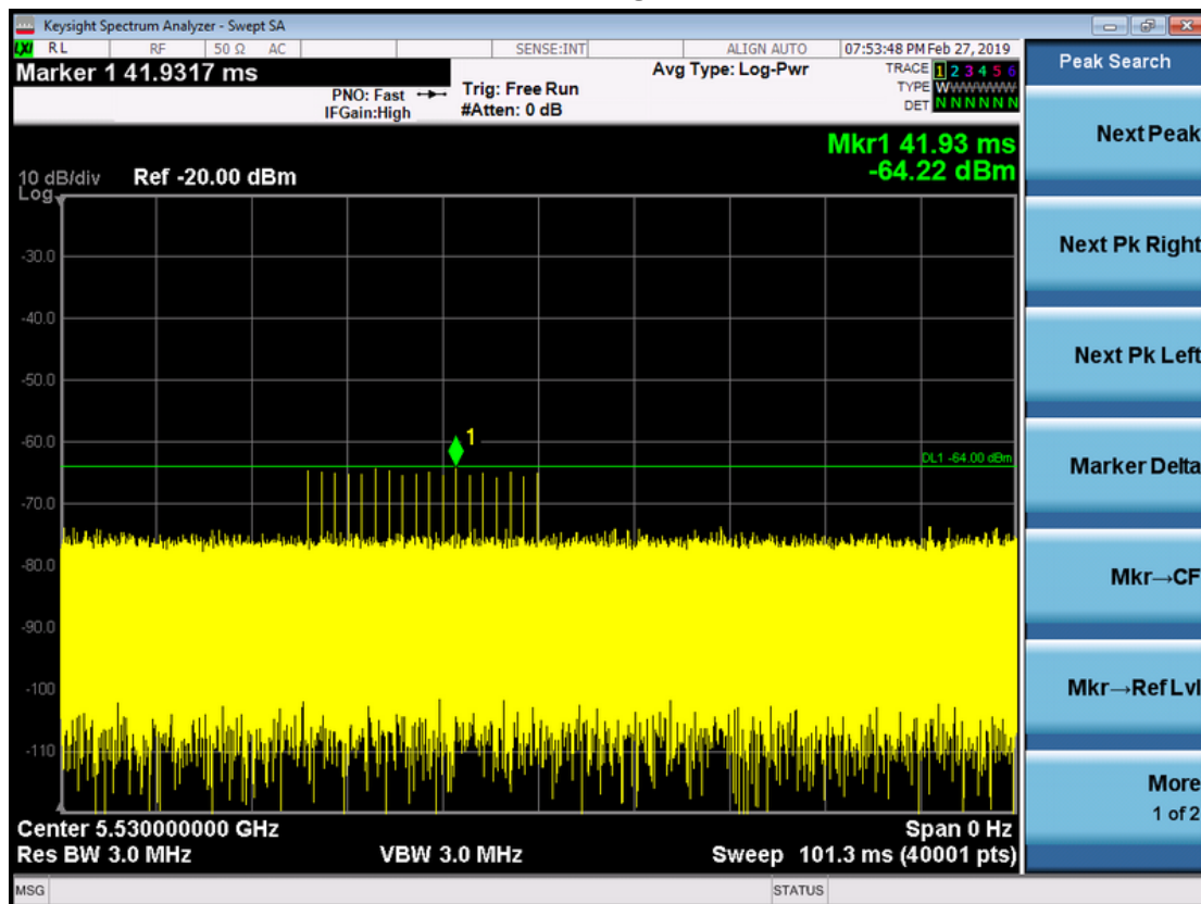
Radar Signal 0
