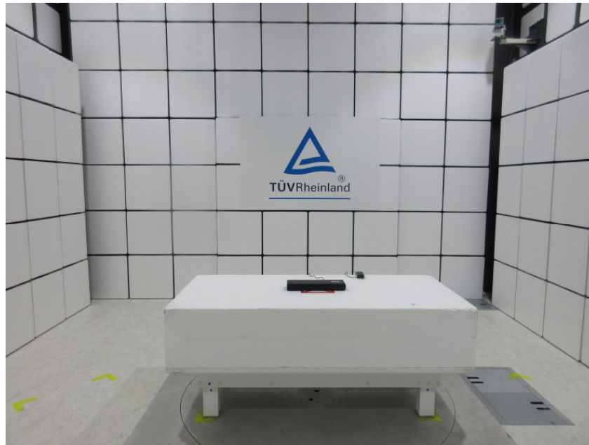
Photograph 1: Set-up for Spurious Emissions (Front View 1)
