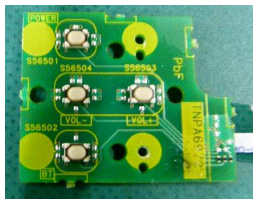
BUTTON PCB
