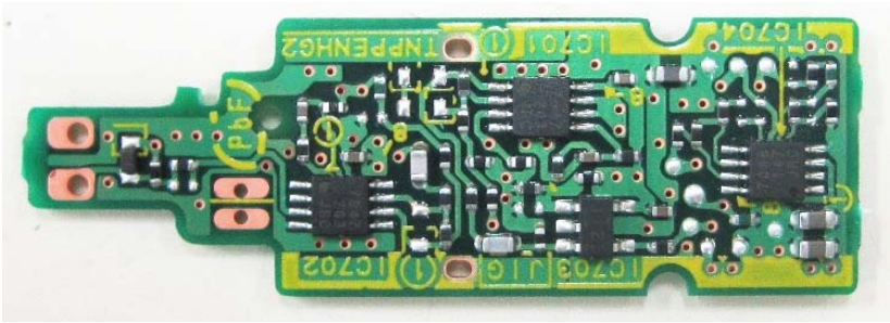
4)-2 Circuit Pen Top (top, without shielding)
