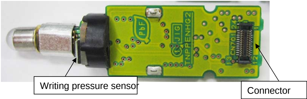
4)-3 Circuit Pen Top (bottom)
