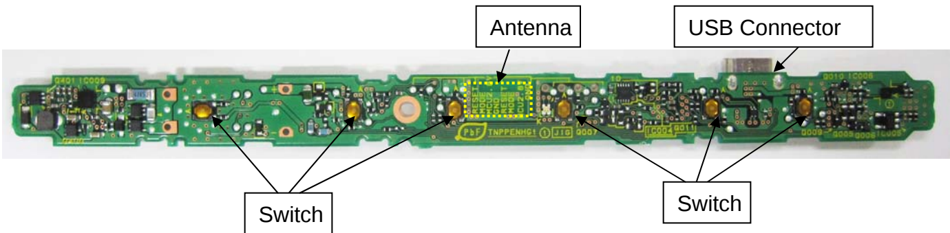
6)-1 Circuit Main (top)
