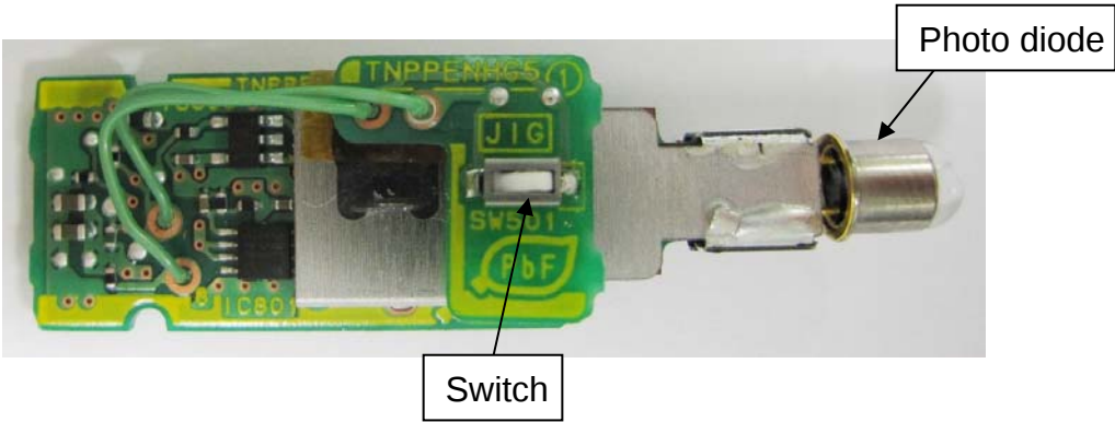
5)-1 Circuit Eraser Top (top)
