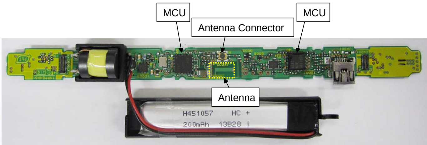
6)-2 Circuit Main (bottom)
