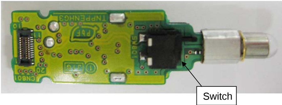
5)-4 Circuit Eraser Top (bottom, without shielding)
