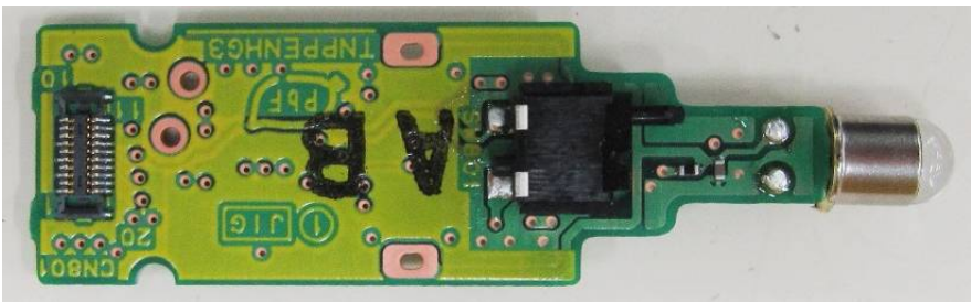
5)-4 Circuit Eraser Top (bottom, without shielding)
