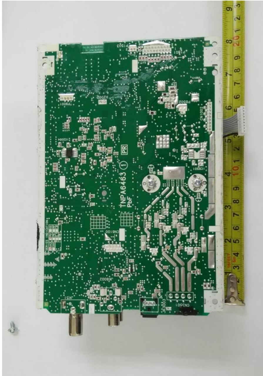
Main PCB Trace Side
