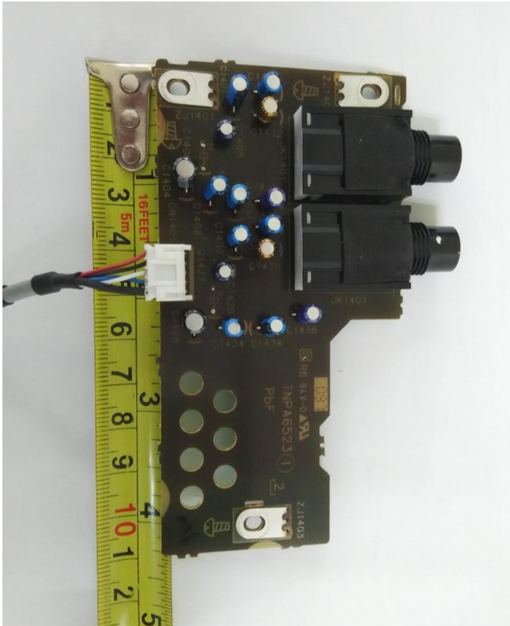
Microphone PCB Component Side
