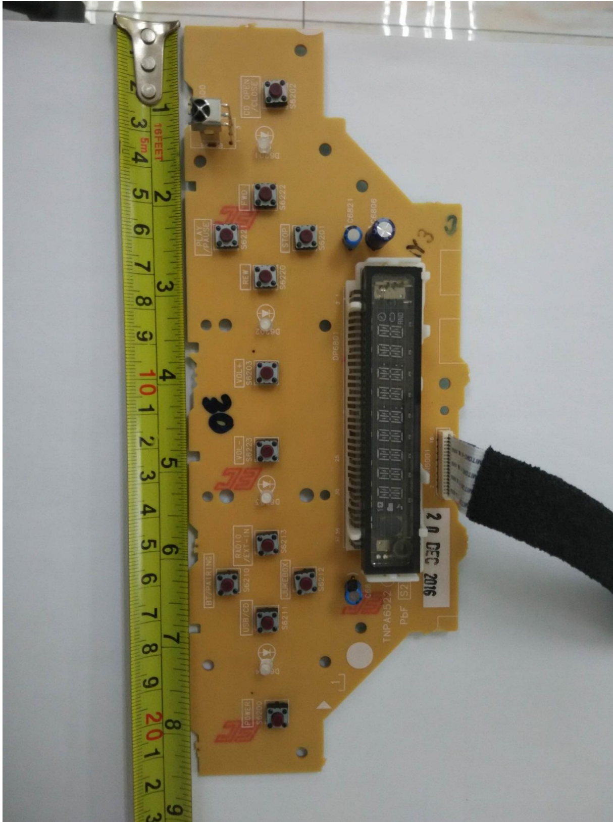
Panel PCB Component Side
