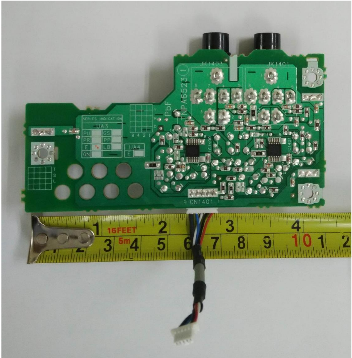
Microphone PCB Trace Side
