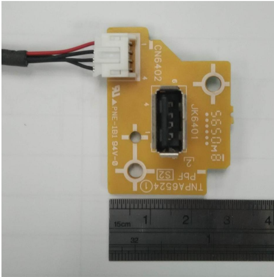
USB PCB Component Side
