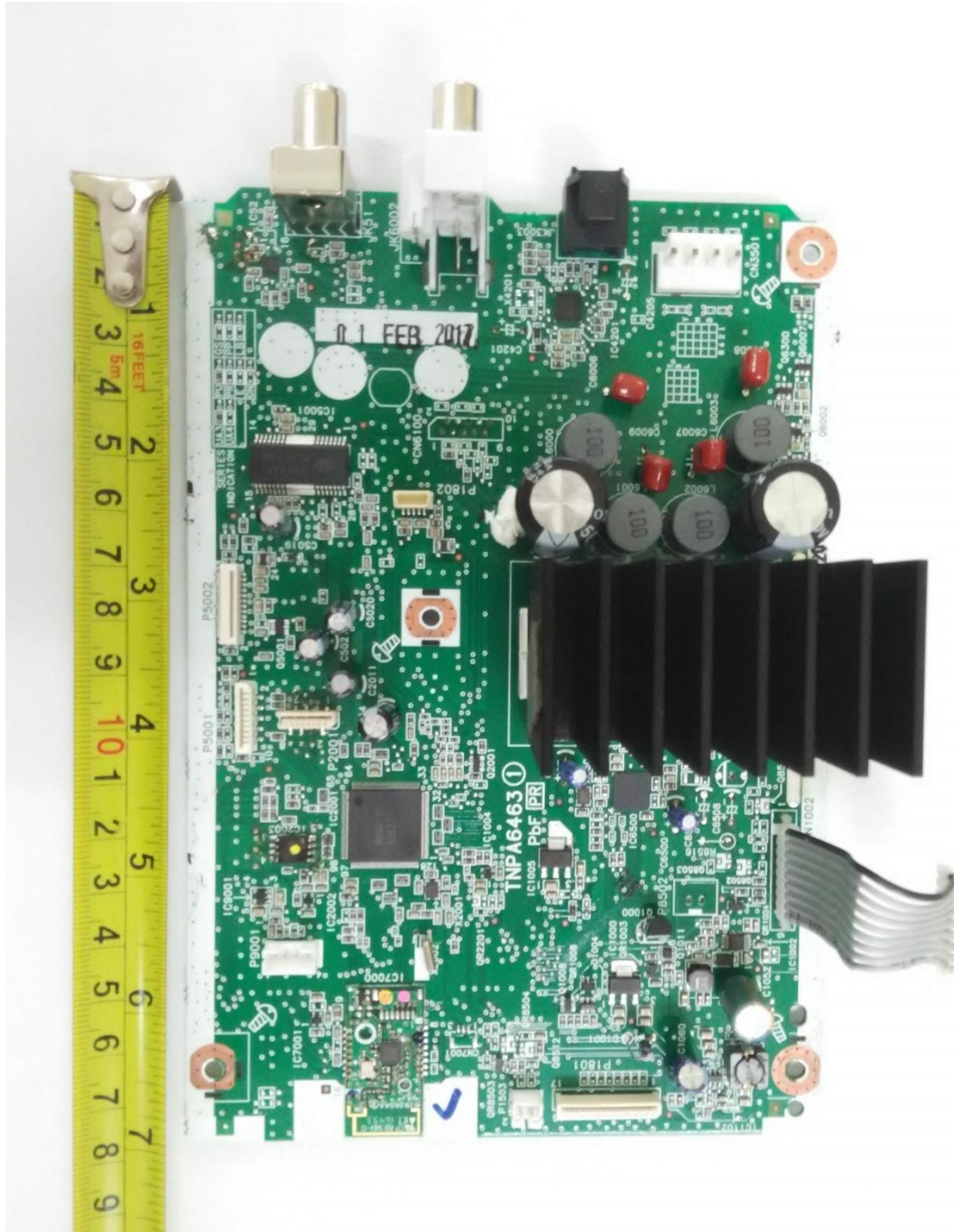
Main PCB Component Side
