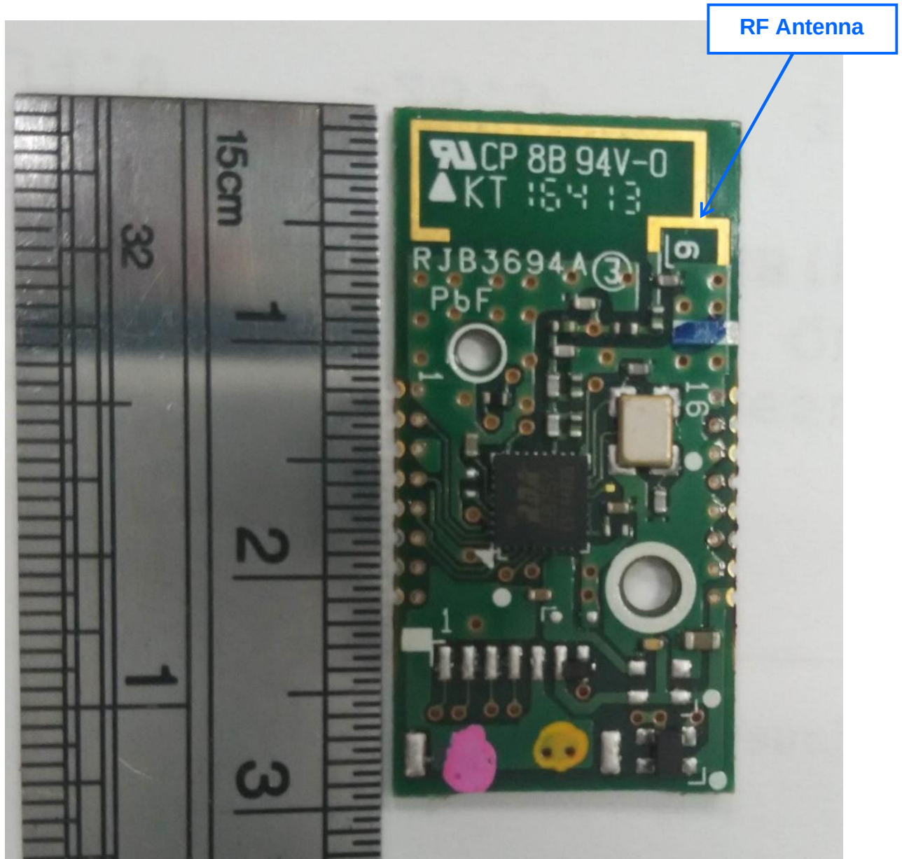
Bluetooth PCB Component Side
