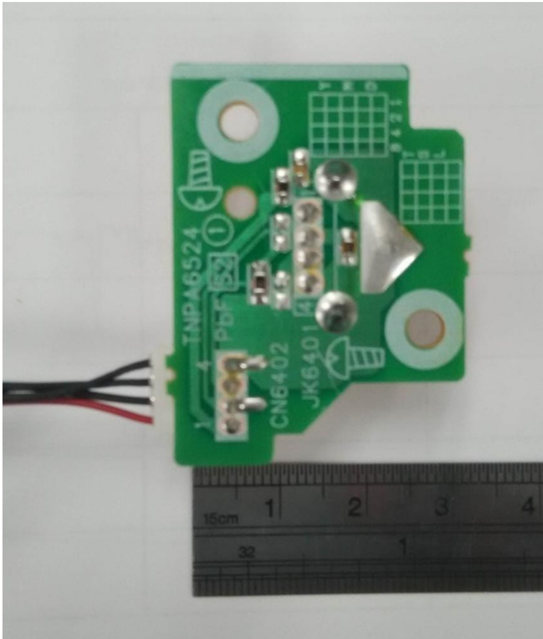
USB PCB Trace Side
