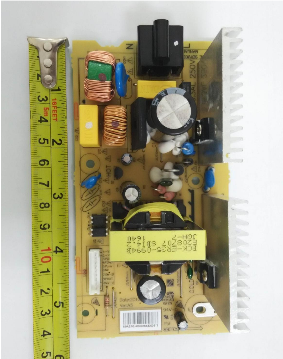
SMPS PCB Component Side
