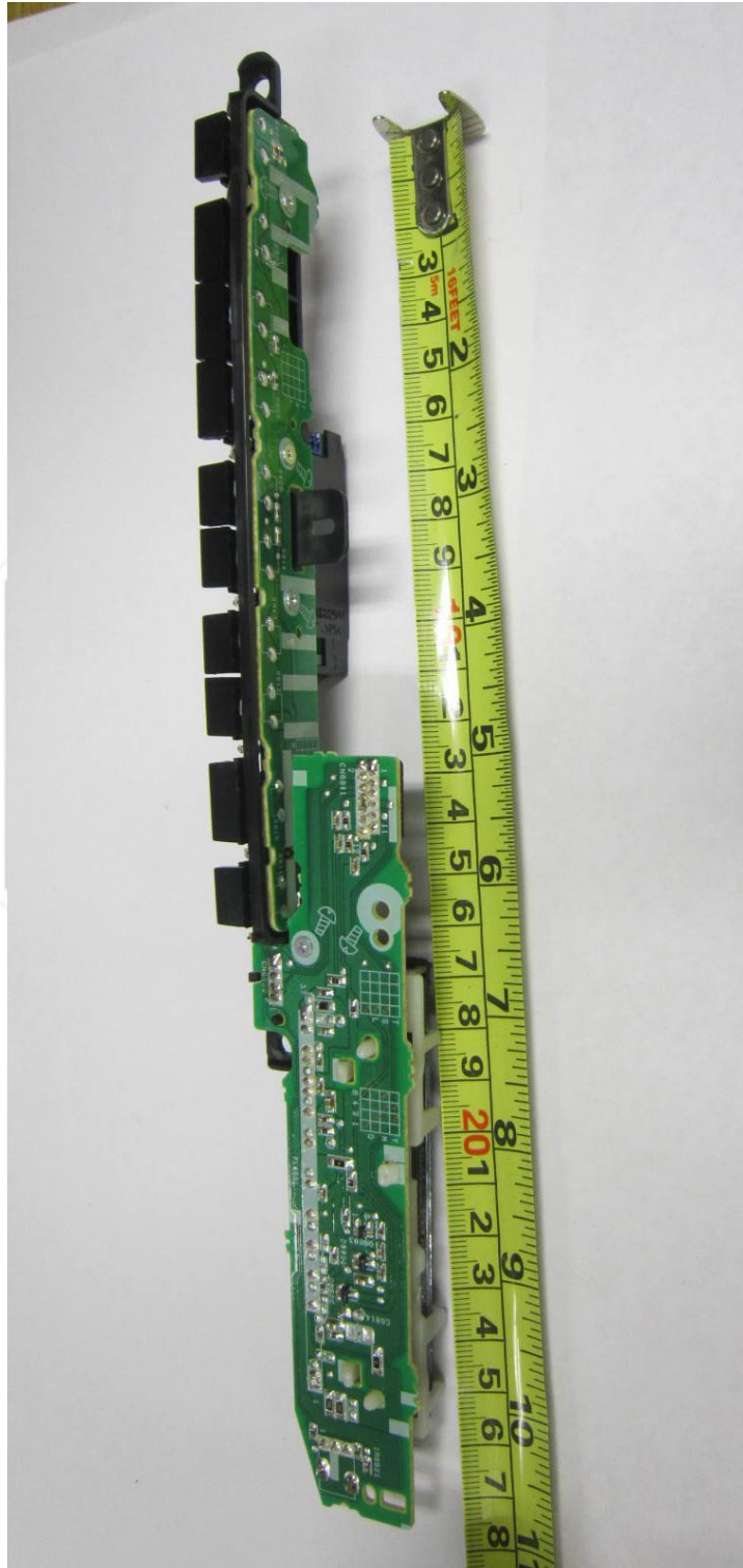
LCD Display Board PCB View 3
