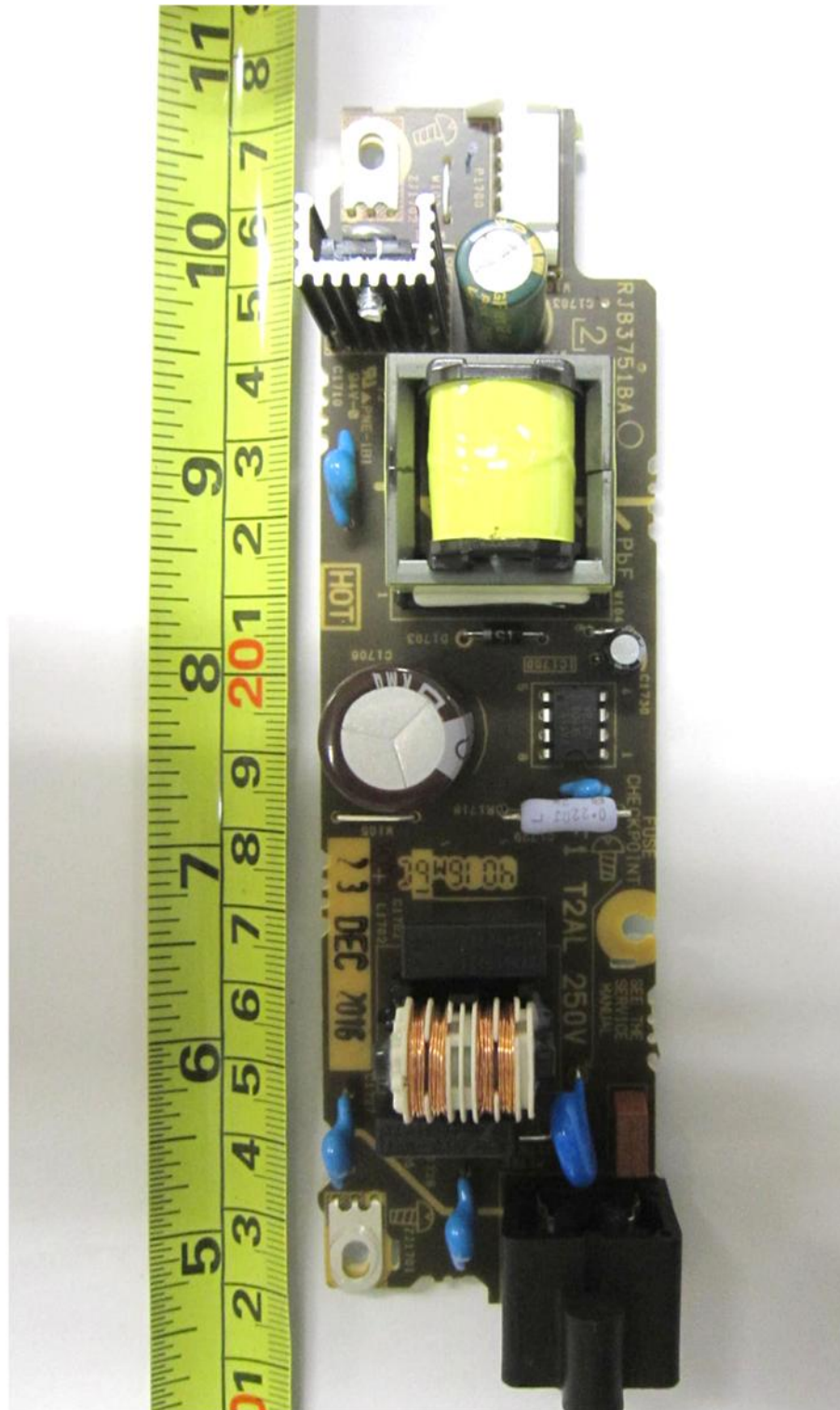
Power Supply Board PCB Component Side
