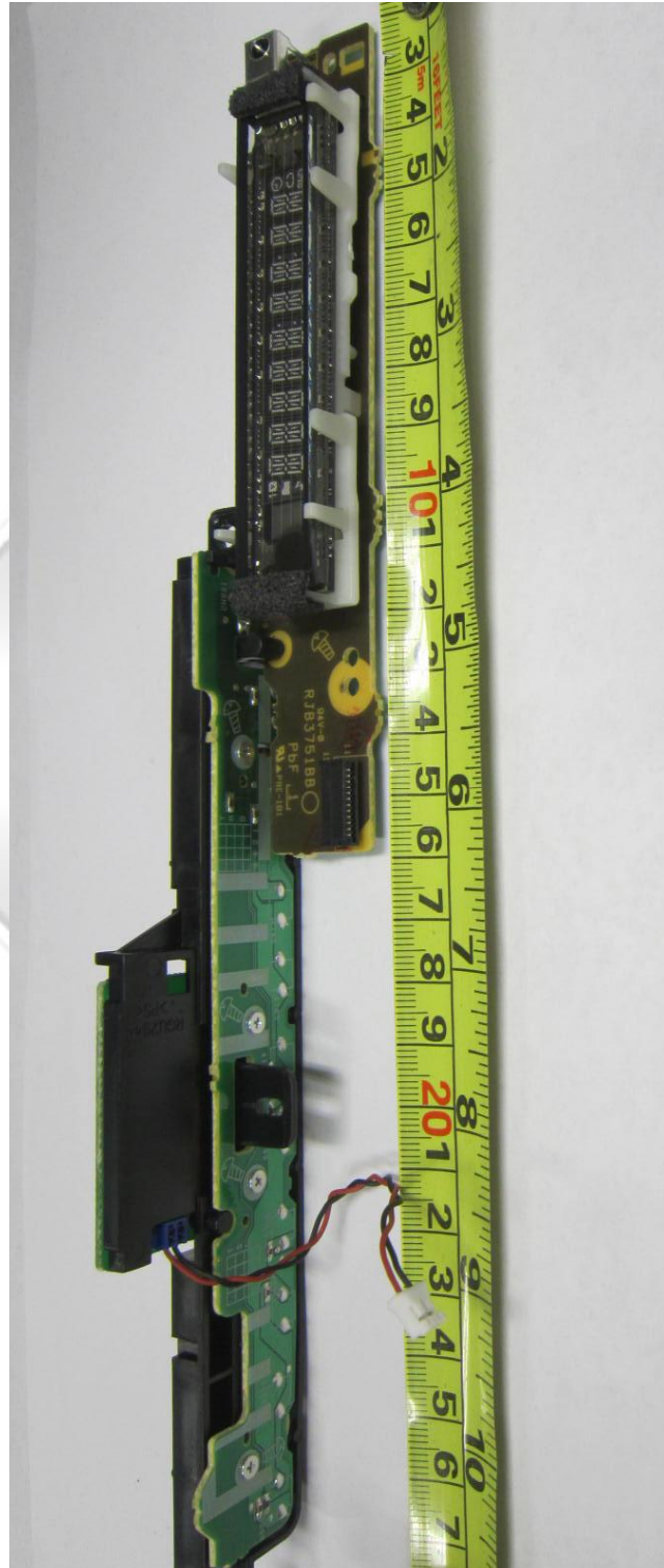
LCD Display Board PCB View 1
