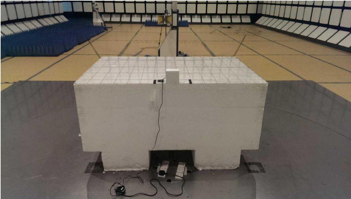
Band Edge Compliance (Radiated) Test Setup
