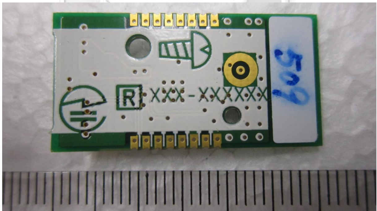
RF Module Circuit Trace Side
