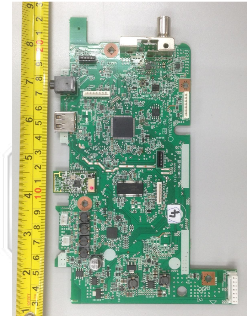
Main-Board PCB Component Side
