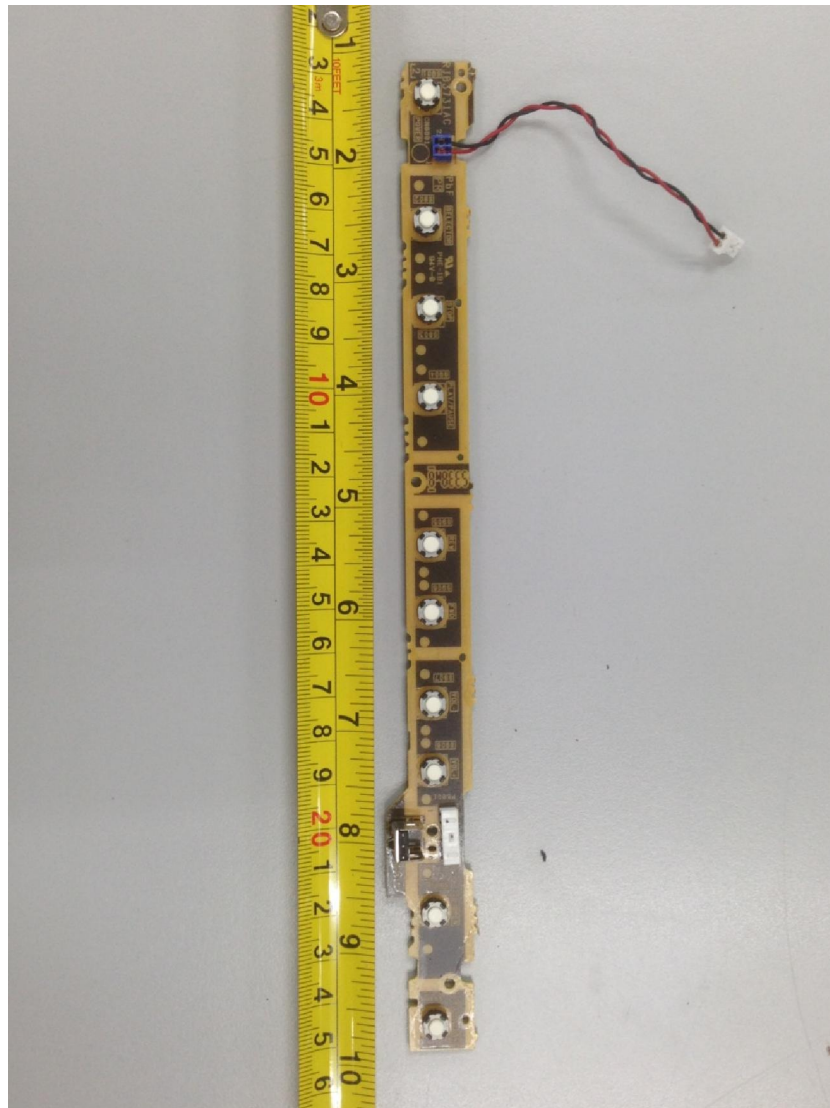
Button PCB Component Side
