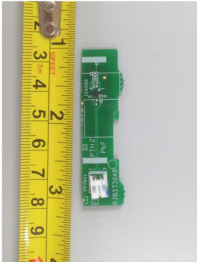
NFC PCB Component Side
