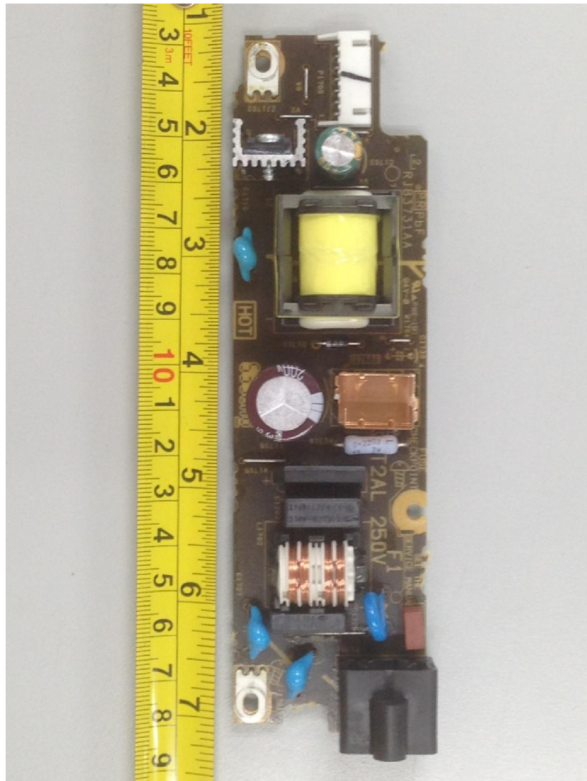
SMPS PCB Component Side
