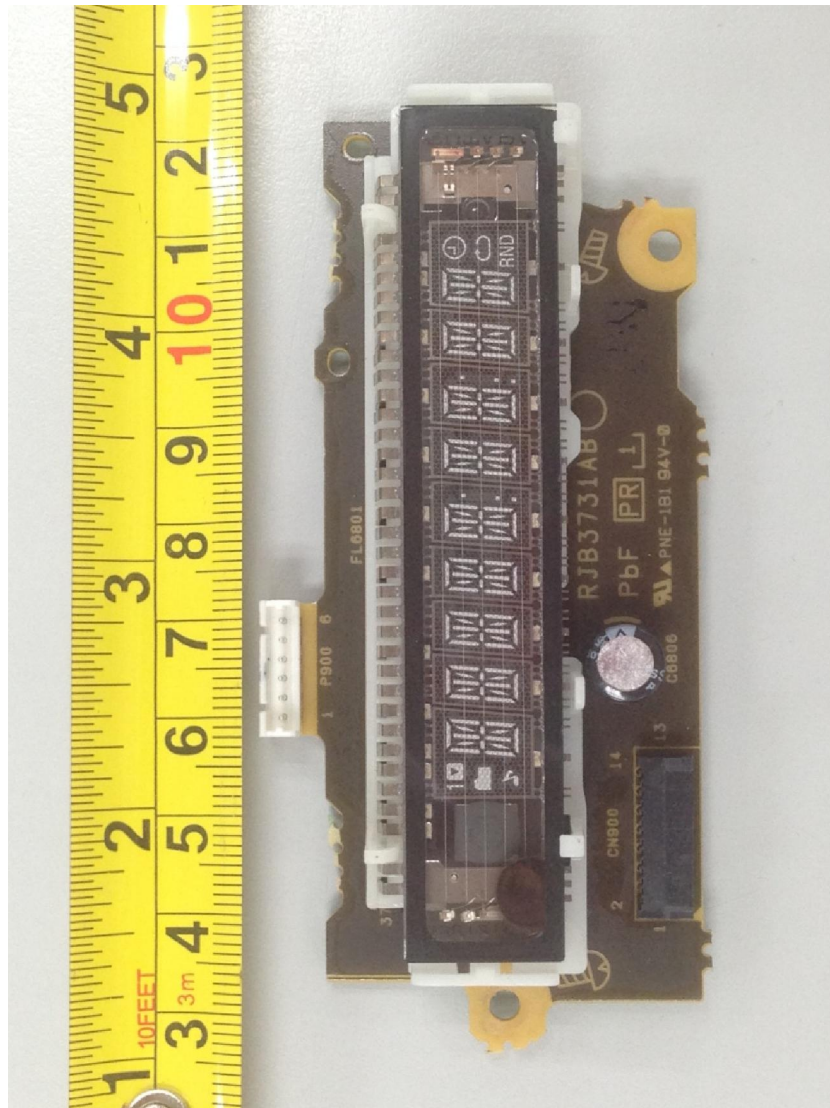
FL PCB Component Side
