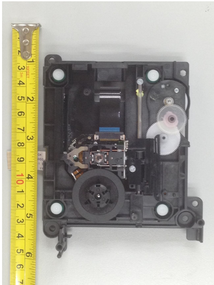
CD Mega PCB Component Side
