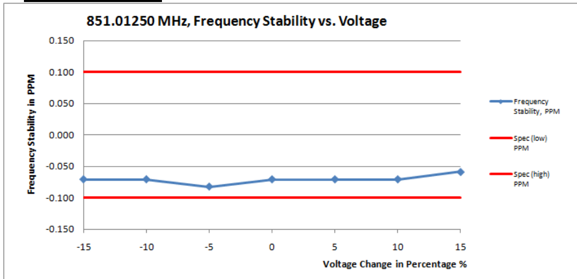
(i) Frequency Stability VS Voltage
