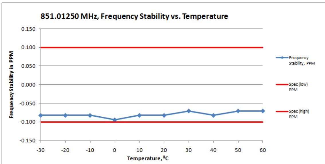
(ii) Frequency Stability VS temperature
