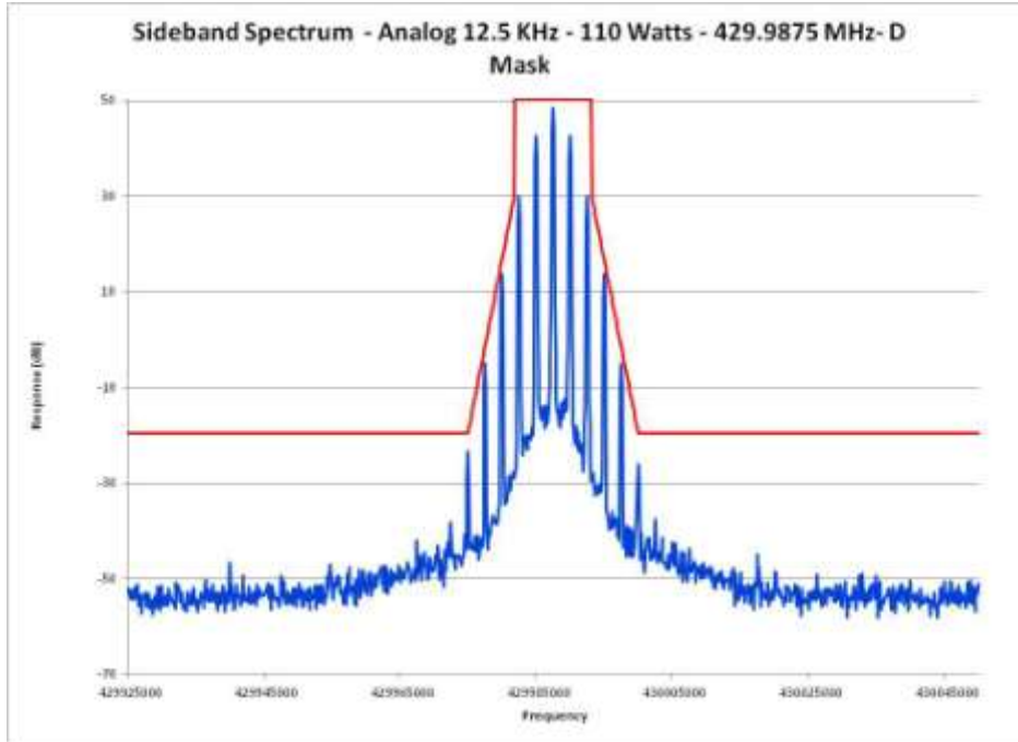
E1-5.31 Occupied Bandwidth, Analog, 12.5 kHz Channels, 429.9875 MHz
