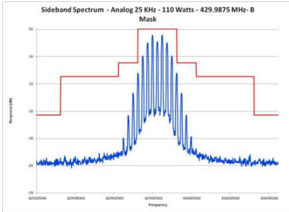
E1-5.13 Occupied Bandwidth, Analog, 25 kHz Channels, 429.9875 MHz
