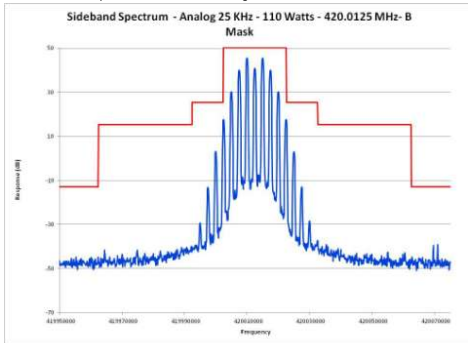
E1-5.10 Occupied Bandwidth, Analog, 25 kHz Channels, 420.0125 MHz
