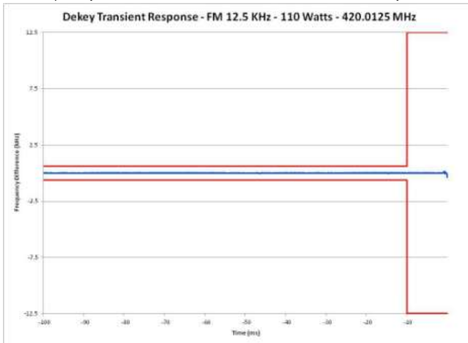
E1-9.20 Frequency Transient Behavior, 12.5 kHz Channel De-key, 420.0125 MHz
