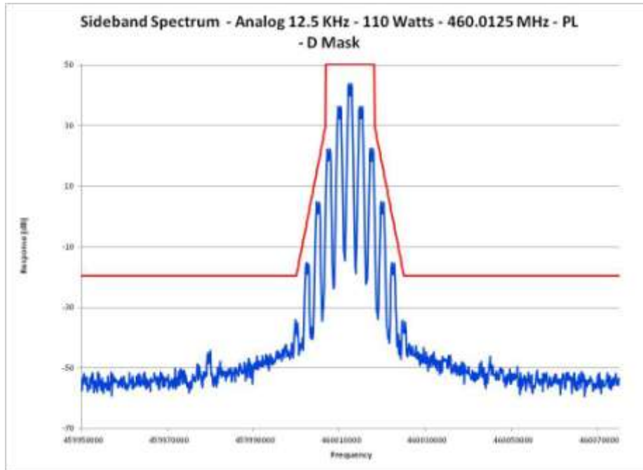
E1-5.38 Occupied Bandwidth, Analog, 12.5 kHz Channels, 460.0125 MHz PL
