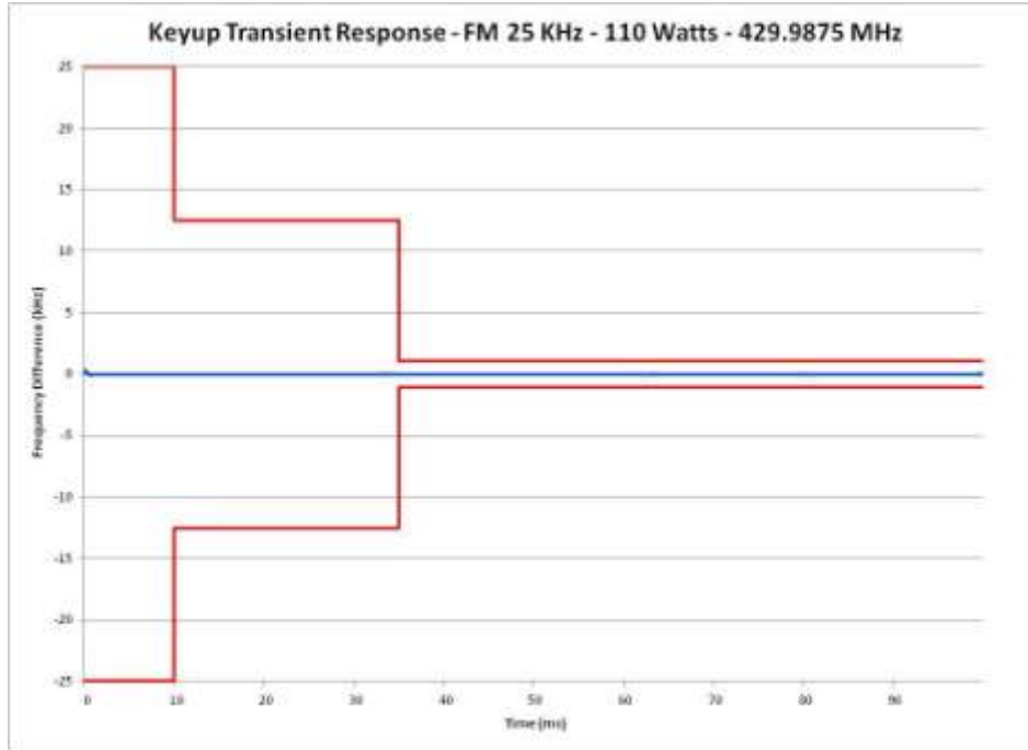
E1-9.3 Frequency Transient Behavior, 25 kHz Channel Key-Up, 429.9875MHz
