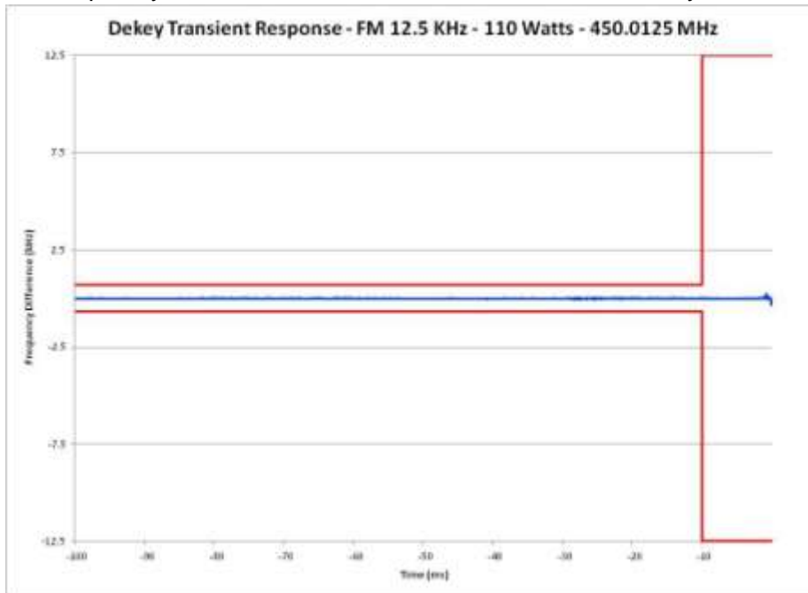
E1-9.22 Frequency Transient Behavior, 12.5 kHz Channel De-key, 450.0125 MHz
