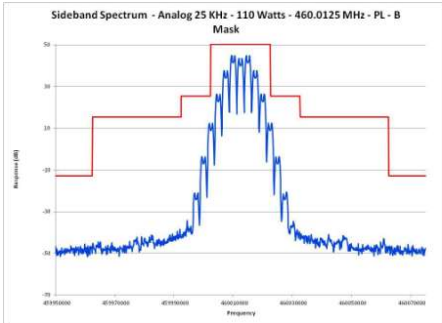
E1-5.20 Occupied Bandwidth, Analog, 25 kHz Channels, 460.0125 MHz PL
