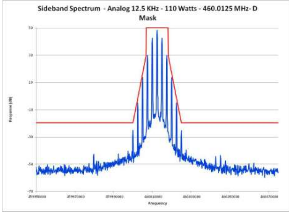
E1-5.37 Occupied Bandwidth, Analog, 12.5 kHz Channels, 460.0125 MHz
