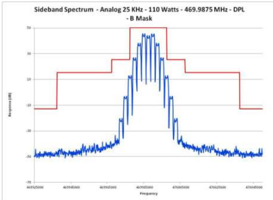
E1-5.24 Occupied Bandwidth, Analog, 25 kHz Channels, 469.9875 MHz DPL
