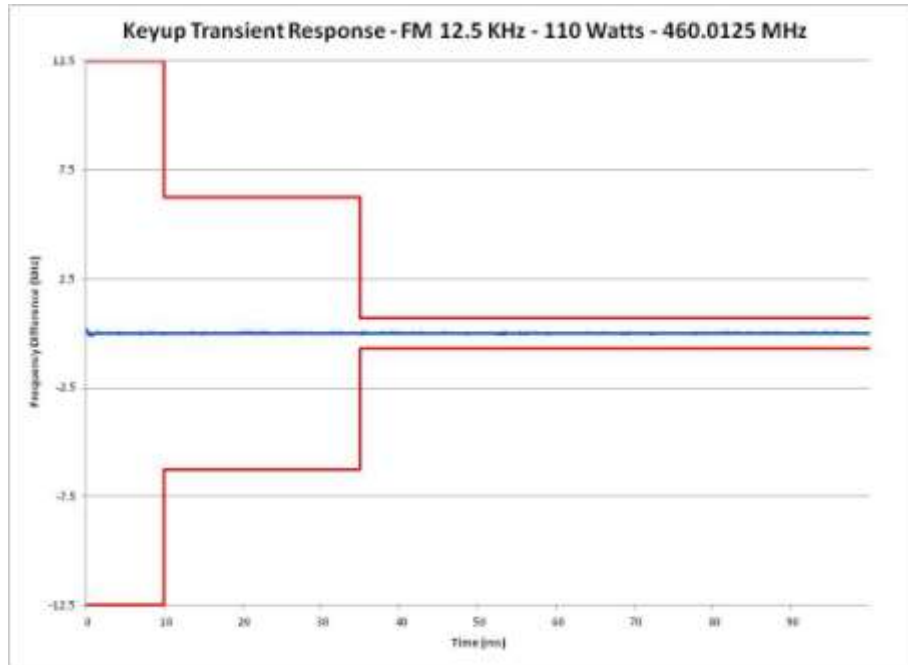
E1-9.17 Frequency Transient Behavior, 12.5 kHz Channel Key-Up, 460.0125 MHz
