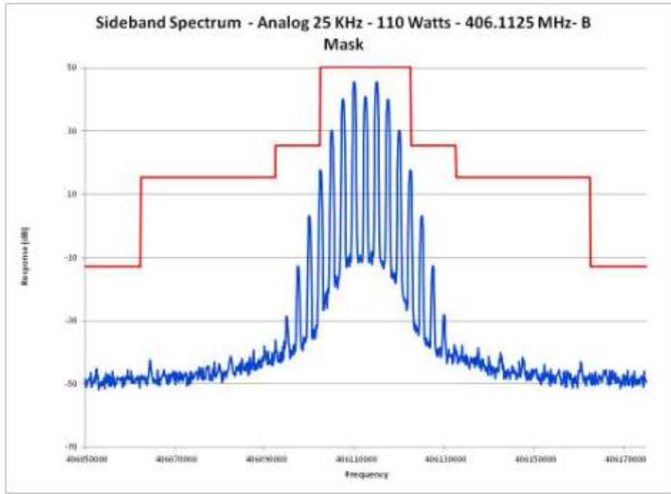
E1-5.7 Occupied Bandwidth, Analog, 25 kHz Channels, 406.1125 MHz
