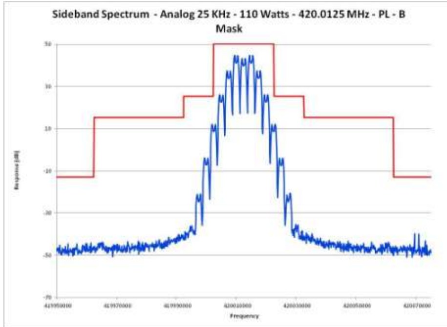
E1-5.11 Occupied Bandwidth, Analog, 25 kHz Channels, 420.0125 MHz PL
