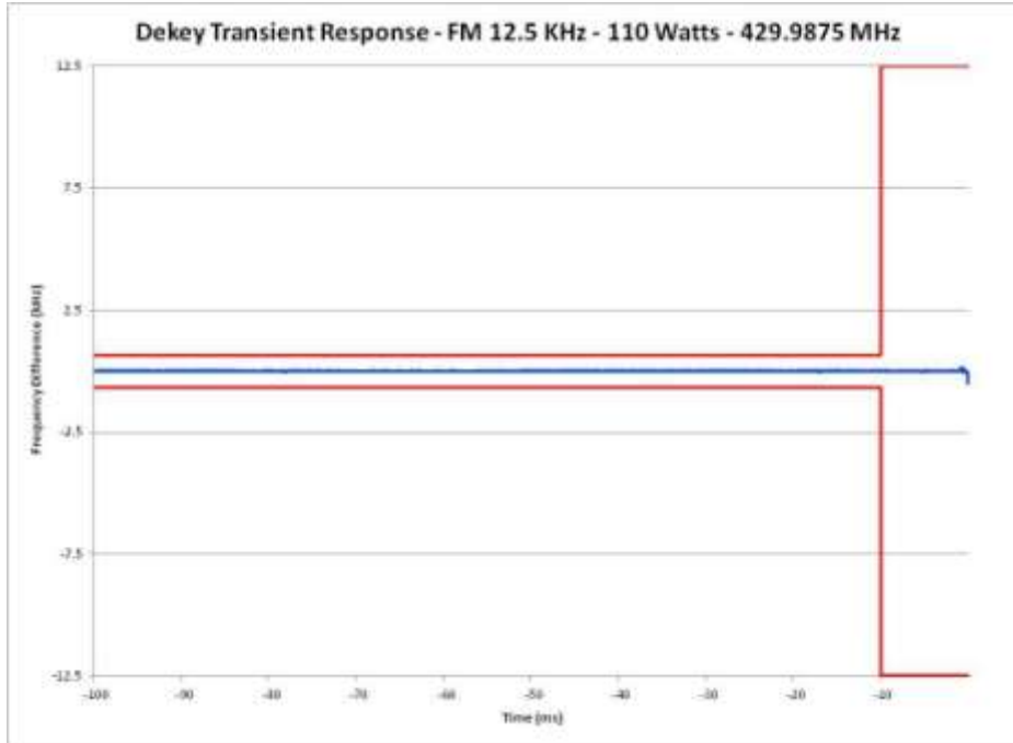
E1-9.21 Frequency Transient Behavior, 12.5 kHz Channel De-key, 429.9875 MHz
