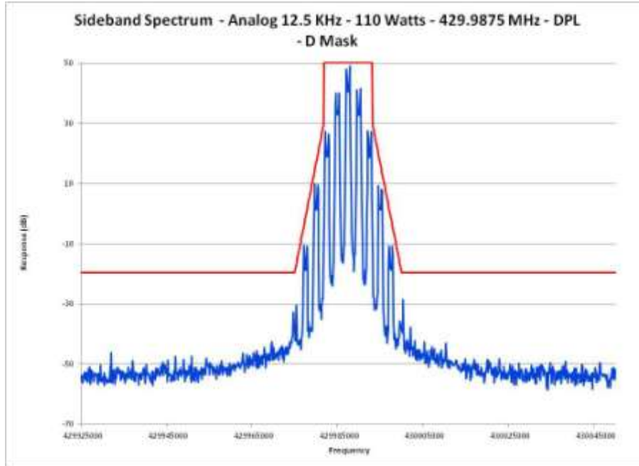
E1-5.33 Occupied Bandwidth, Analog, 12.5 kHz Channels, 429.9875 MHz DPL
