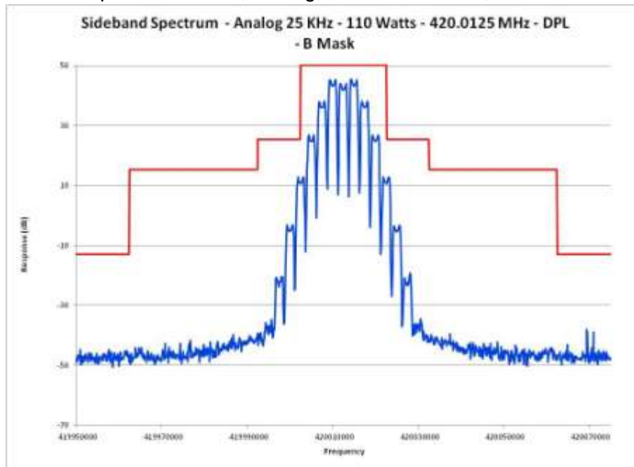
E1-5.12 Occupied Bandwidth, Analog, 25 kHz Channels, 420.0125 MHz DPL
