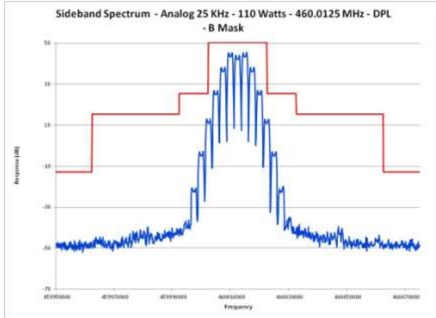
E1-5.21 Occupied Bandwidth, Analog, 25 kHz Channels, 460.0125 MHz DPL
