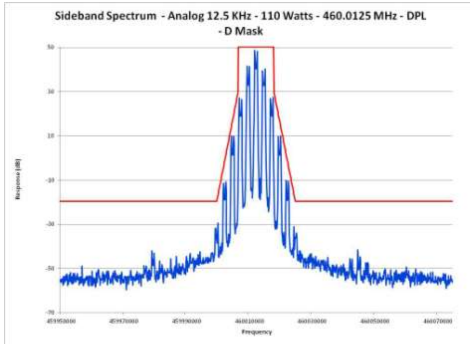
E1-5.39 Occupied Bandwidth, Analog, 12.5 kHz Channels, 460.0125 MHz DPL
