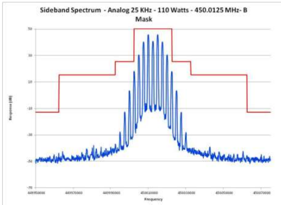
E1-5.17 Occupied Bandwidth, Analog, 25 kHz Channels, 450.0125 MHz PL
