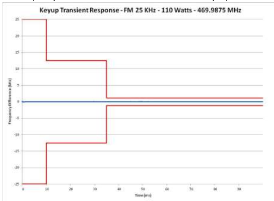
E1-9.6 Frequency Transient Behavior, 25 kHz Channel Key-Up, 469.9875 MHz
