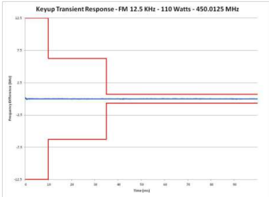
E1-9.16 Frequency Transient Behavior, 12.5 kHz Channel Key-Up, 450.0125 MHz
