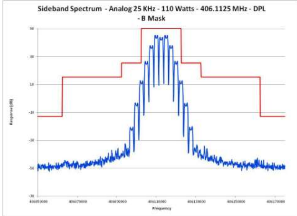
E1-5.9 Occupied Bandwidth, Analog, 25 kHz Channels, 406.1125 MHz DPL
