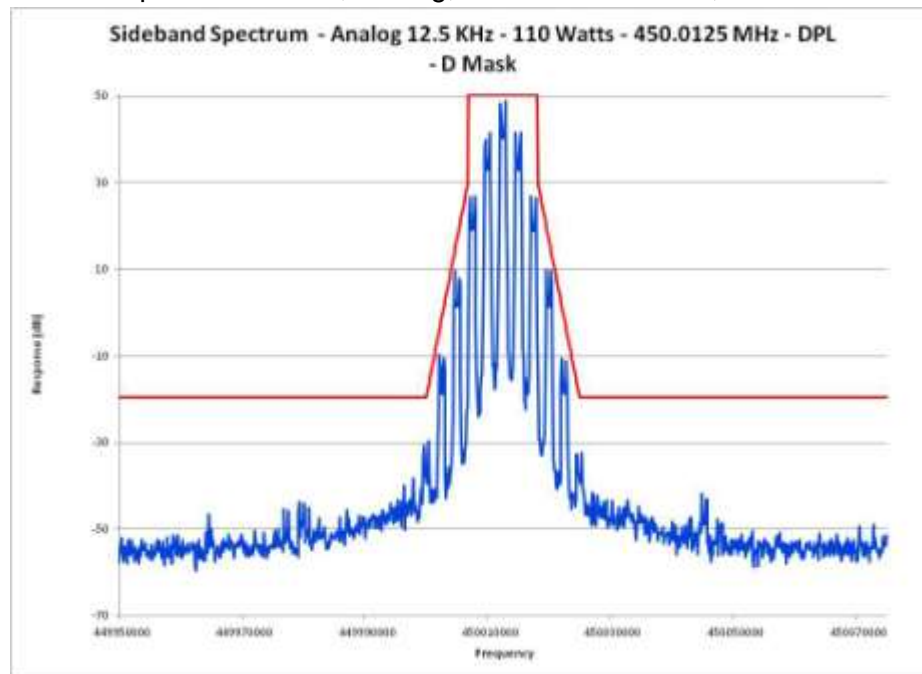
E1-5.36 Occupied Bandwidth, Analog, 12.5 kHz Channels, 450.0125 MHz DPL
