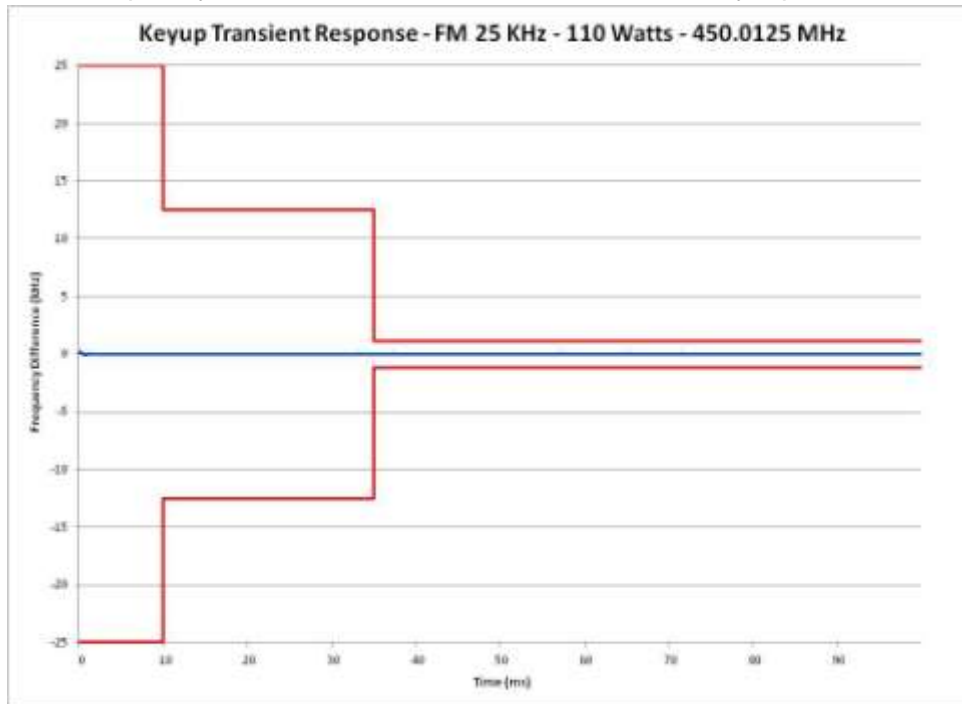
E1-9.4 Frequency Transient Behavior, 25 kHz Channel Key-Up, 450.0125 MHz
