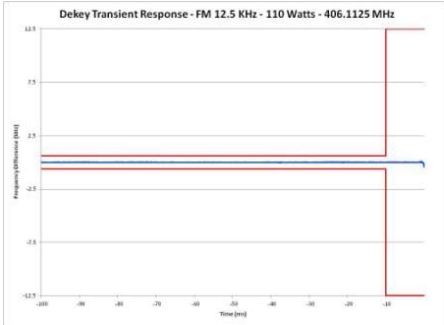
E1-9.19 Frequency Transient Behavior, 12.5 kHz Channel De-key, 406.1125 MHz
