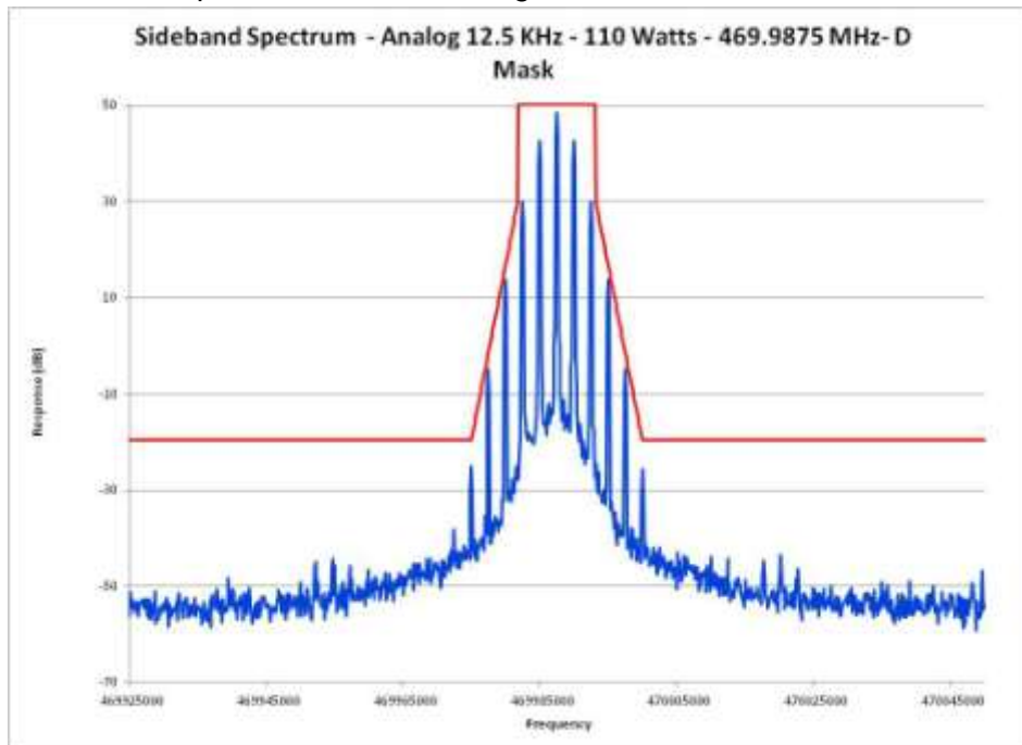
E1-5.40 Occupied Bandwidth, Analog, 12.5 kHz Channels, 469.9875 MHz
