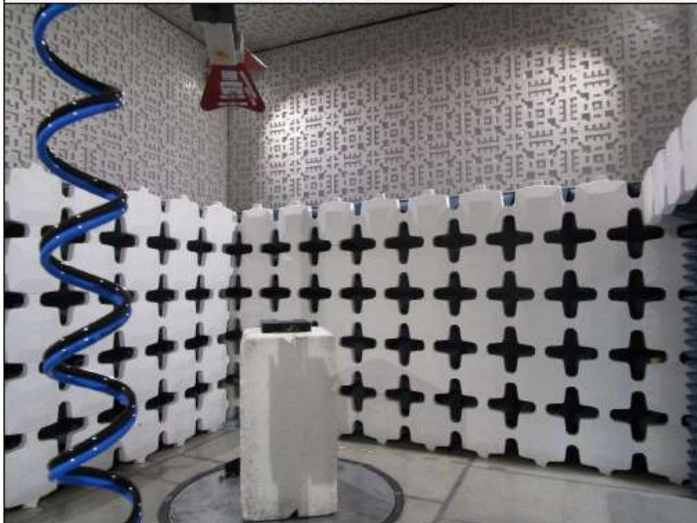
Test Setup for Spurious Radiated Emissions, Above 1GHz – Antenna Polarization
