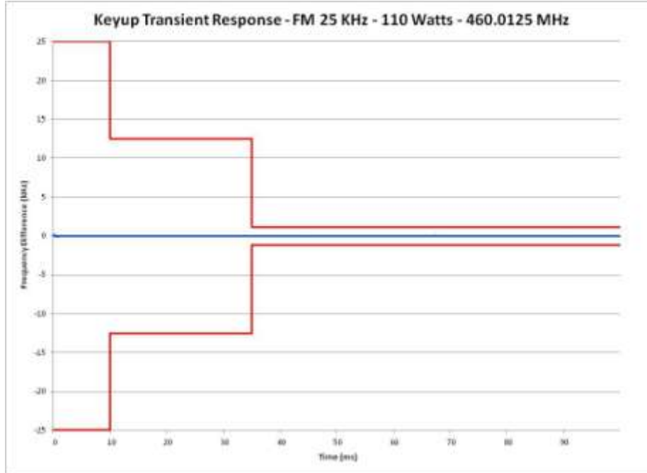
E1-9.5 Frequency Transient Behavior, 25 kHz Channel Key-Up, 460.0125 MHz
