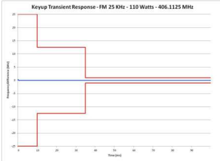
E1-9.1 Frequency Transient Behavior, 25 kHz Channel Key-Up, 406.1125MHz
