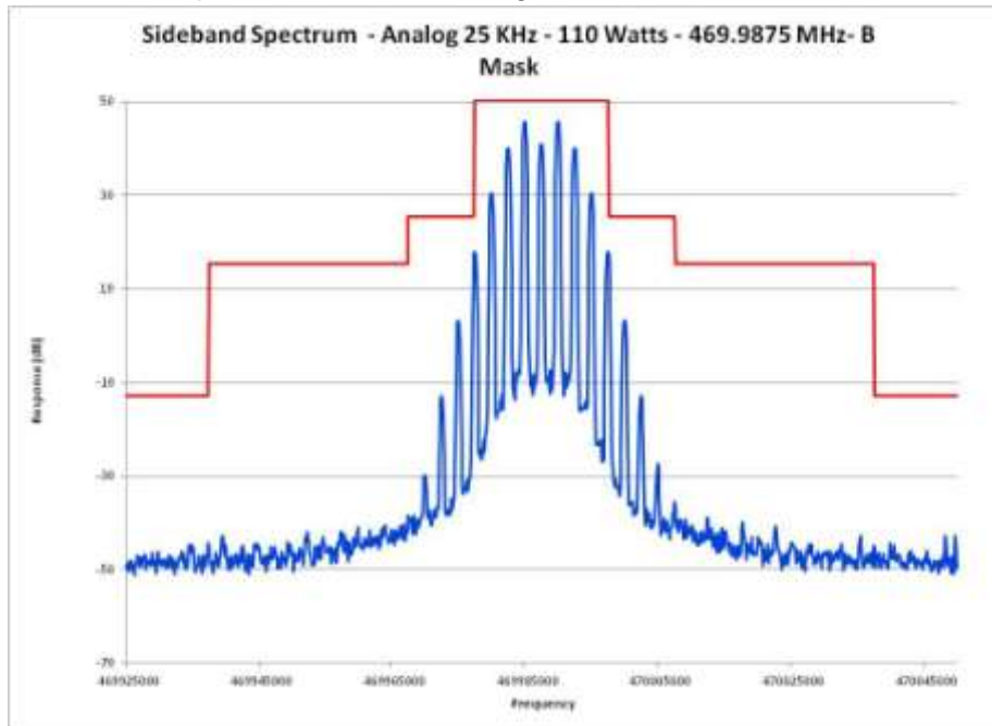
E1-5.22 Occupied Bandwidth, Analog, 25 kHz Channels, 469.9875 MHz
