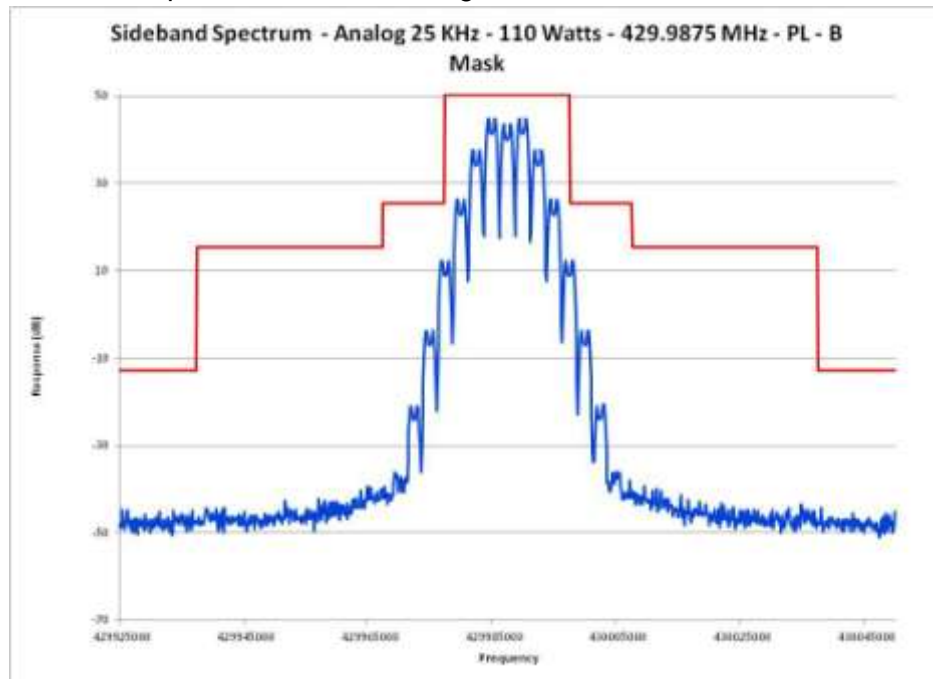
E1-5.14 Occupied Bandwidth, Analog, 25 kHz Channels, 429.9875 MHz PL
