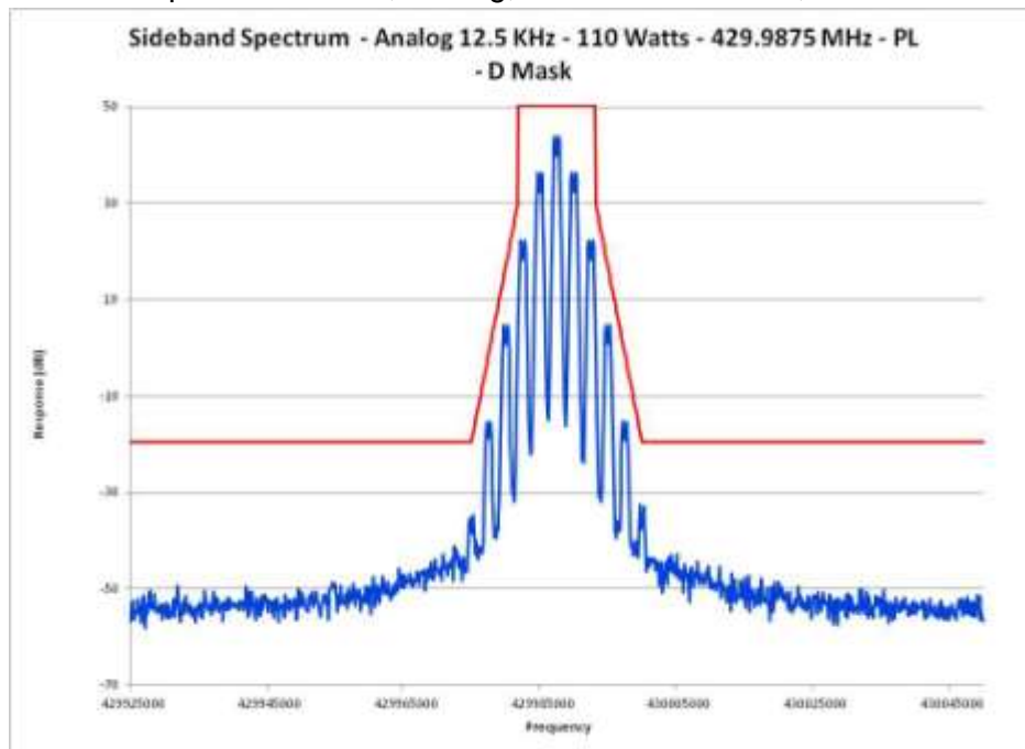
E1-5.32 Occupied Bandwidth, Analog, 12.5 kHz Channels, 429.9875 MHz PL
