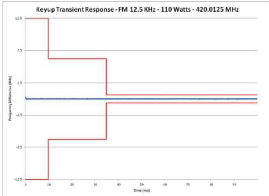
E1-9.14 Frequency Transient Behavior, 12.5 kHz Channel Key-Up, 420.0125 MHz
