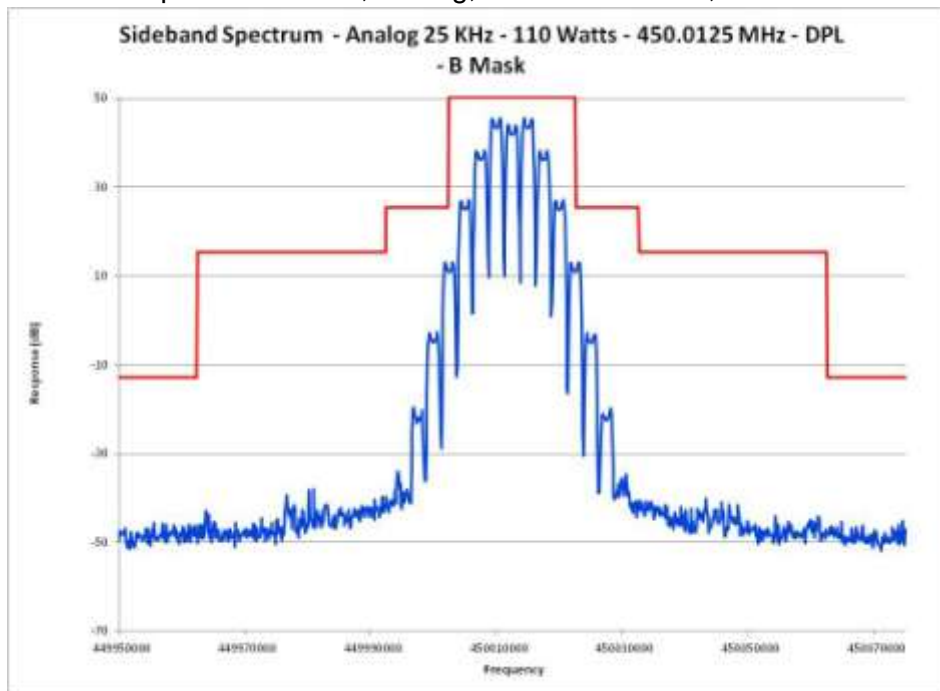
E1-5.18 Occupied Bandwidth, Analog, 25 kHz Channels, 450.0125 MHz DPL
