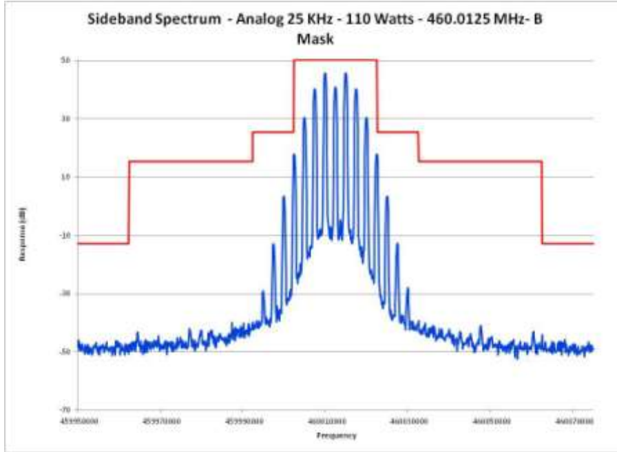
E1-5.19 Occupied Bandwidth, Analog, 25 kHz Channels, 460.0125 MHz
