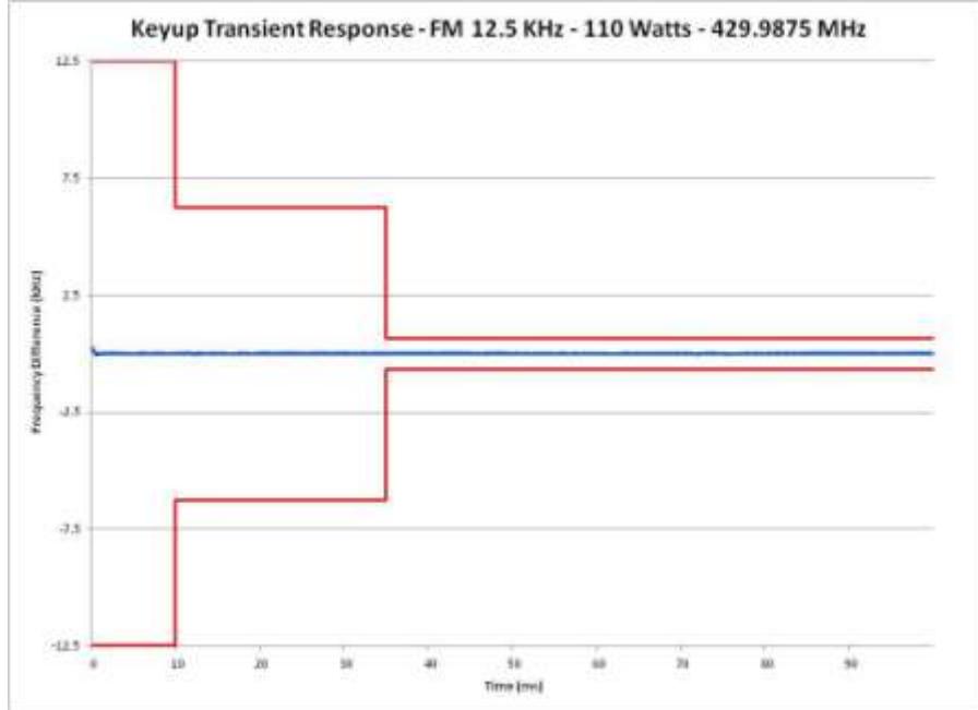
E1-9.15 Frequency Transient Behavior, 12.5 kHz Channel Key-Up, 429.9875 MHz
