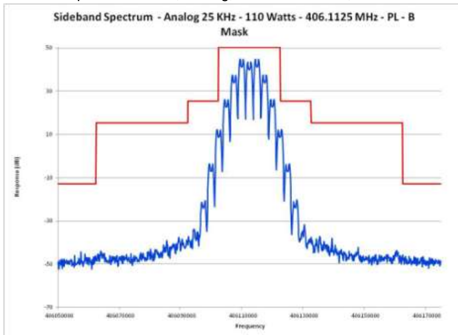
E1-5.8 Occupied Bandwidth, Analog, 25 kHz Channels, 406.1125 MHz PL
