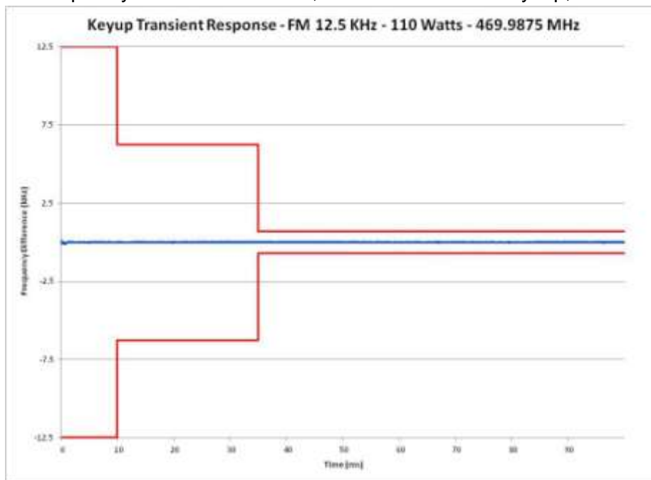
E1-9.18 Frequency Transient Behavior, 12.5 kHz Channel Key-Up, 469.9875 MHz
