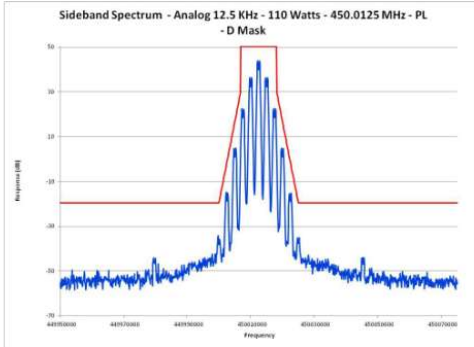
E1-5.35 Occupied Bandwidth, Analog, 12.5 kHz Channels, 450.0125 MHz PL
