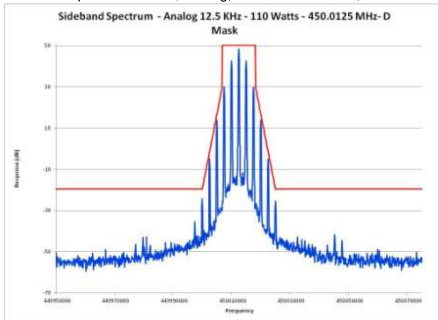
E1-5.34 Occupied Bandwidth, Analog, 12.5 kHz Channels, 450.0125 MHz
