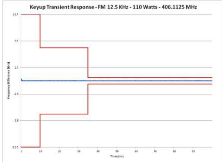
E1-9.13 Frequency Transient Behavior, 12.5 kHz Channel Key-Up, 406.1125 MHz
