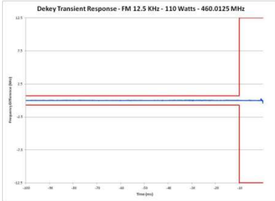
E1-9.23 Frequency Transient Behavior, 12.5 kHz Channel De-key, 460.0125 MHz
