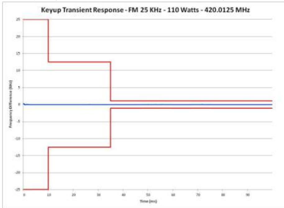
E1-9.2 Frequency Transient Behavior, 25 kHz Channel Key-Up, 420.0125MHz
