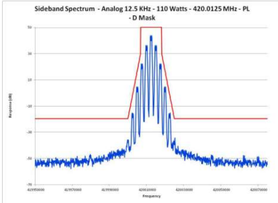
E1-5.29 Occupied Bandwidth, Analog, 12.5 kHz Channels, 420.0125 MHz PL
