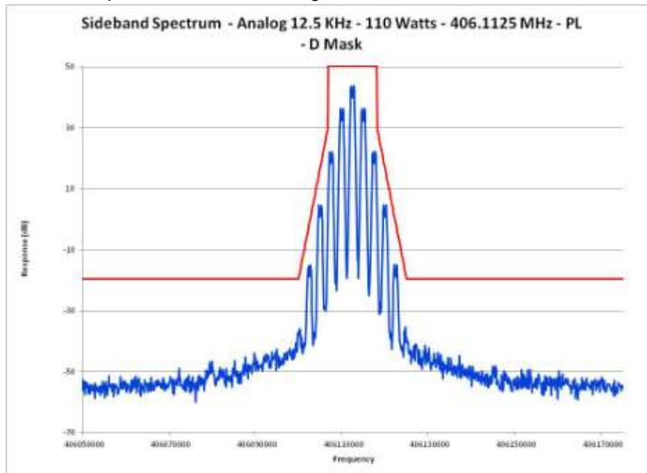
E1-5.26 Occupied Bandwidth, Analog, 12.5 kHz Channels, 406.1125 MHz PL
