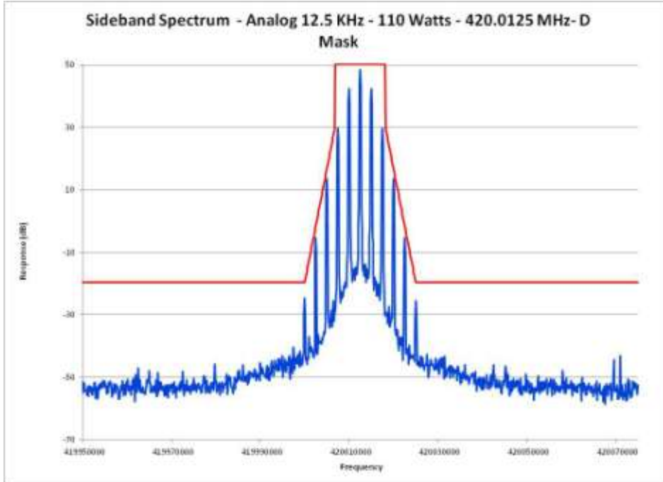
E1-5.28 Occupied Bandwidth, Analog, 12.5 kHz Channels, 420.0125 MHz
