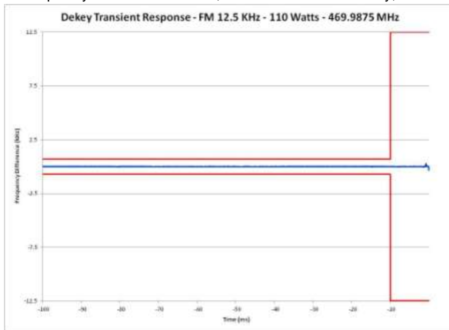
E1-9.24 Frequency Transient Behavior, 12.5 kHz Channel De-key, 469.9875 MHz
