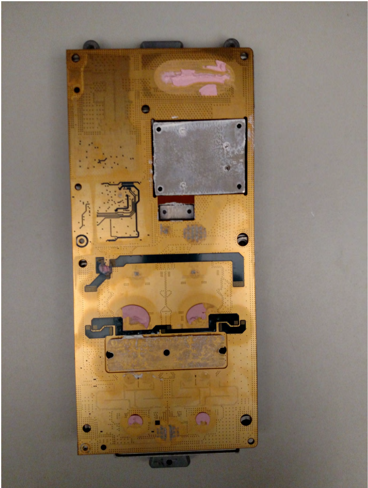
Internal Front View – Power Amplifier Module – Bottom View, Heat Sink Removed
