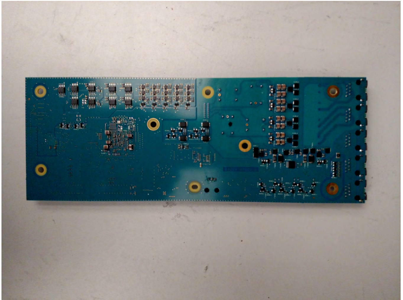
Internal Front View – Wireline Board Bottom View
