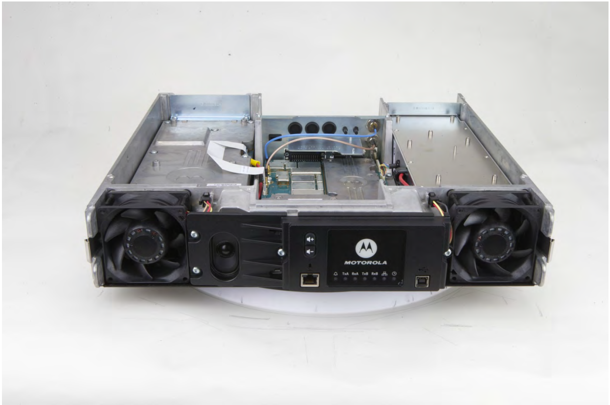
External Front View of Base Radio, Top Cover and Front Panel Removed
