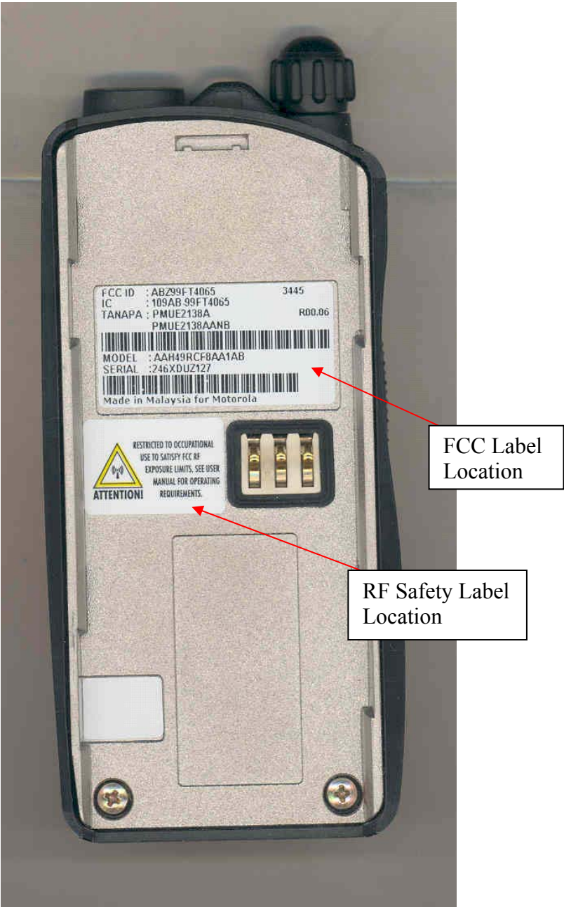
Figure 3-5: Rear view of complete radio showing FCC Label & RF Safety Label location.
