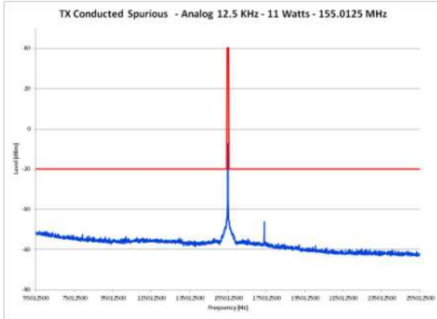
E1-6.5 Conducted Spurious Emission Spectrum, 200 MHz Span, Power 11 Watts, 155.0125MHz
