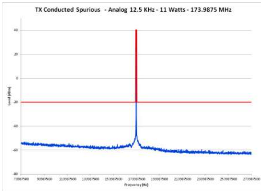
E1-6.6 Conducted Spurious Emission Spectrum, 200 MHz Span, Power 11 Watts, 173.9875MHz
