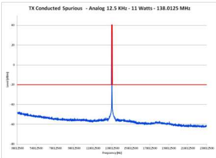
E1-6.4 Conducted Spurious Emission Spectrum, 200 MHz Span, Power 11 Watts, 138.0125MHz
