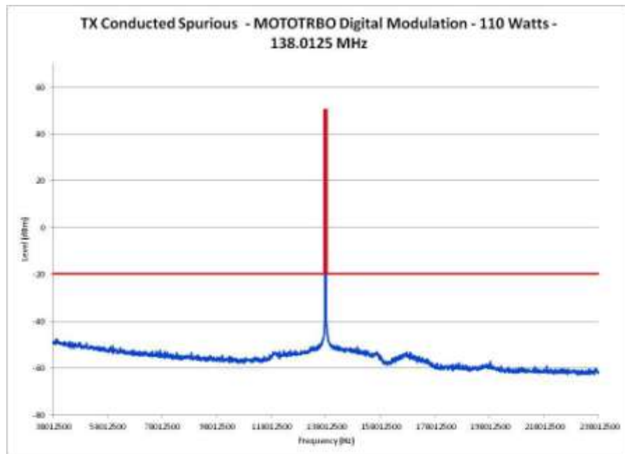
E1-6.4 Conducted Spurious Emission Spectrum, 200 MHz Span, Power 110 Watts, 138.0125MHz
