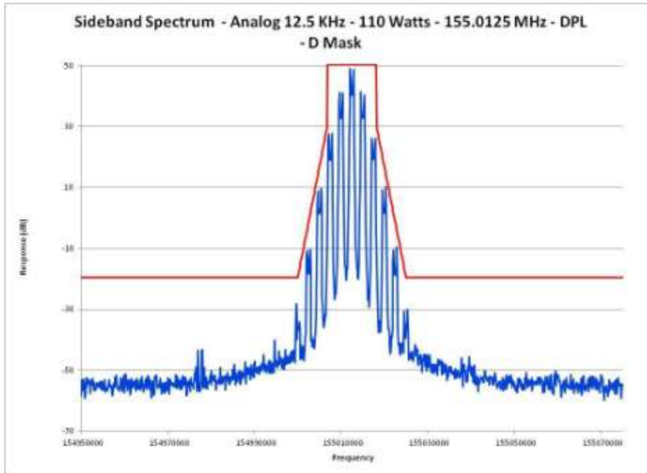
E1-5.25 Occupied Bandwidth, Analog, 12.5 kHz Channels, 155.0125 MHz DPL
