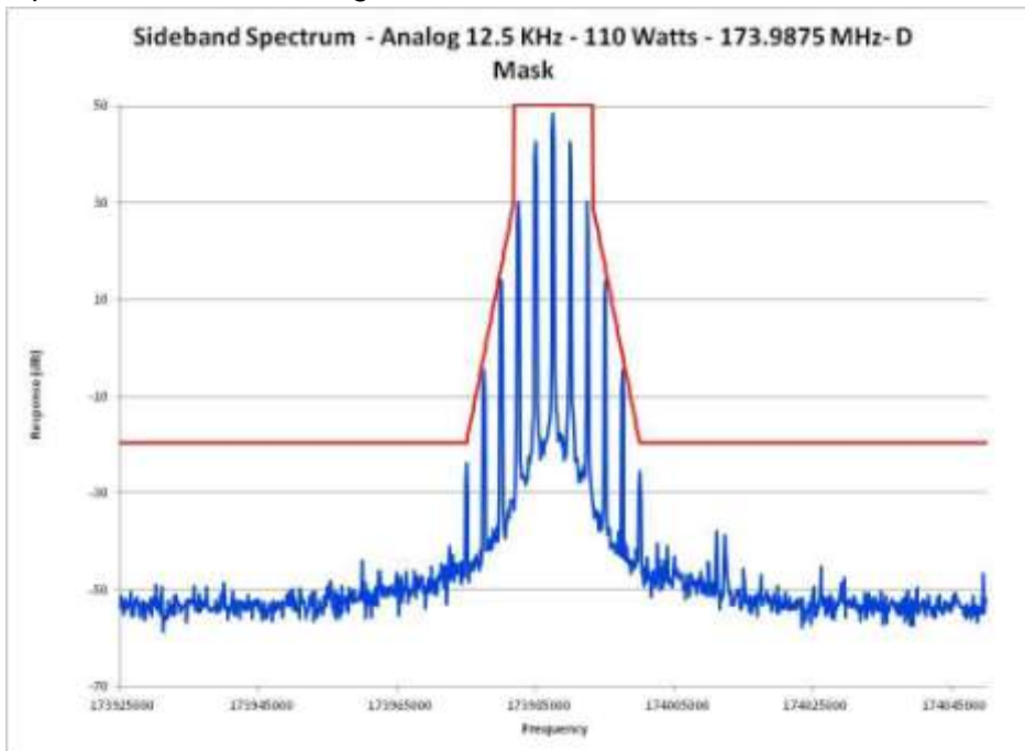
E1-5.26 Occupied Bandwidth, Analog, 12.5 kHz Channels, 173.9875 MHz
