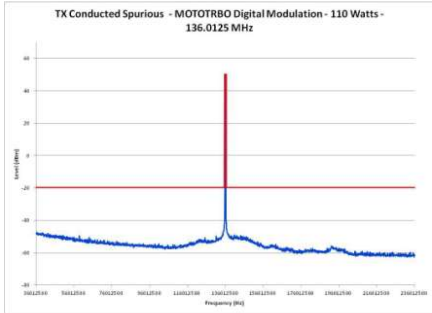
E1-6.3 Conducted Spurious Emission Spectrum, 200 MHz Span, Power 110 Watts, 136.0125MHz
