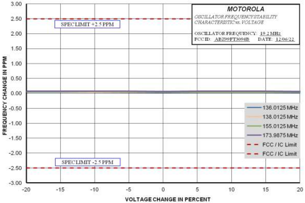
E1-11.2 Frequency Stability Vs Voltage
