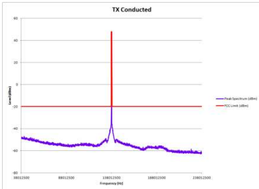
E1-6.4 Conducted Spurious Emission Spectrum, 200 MHz Span, Power 60 Watts, 138.0125MHz
