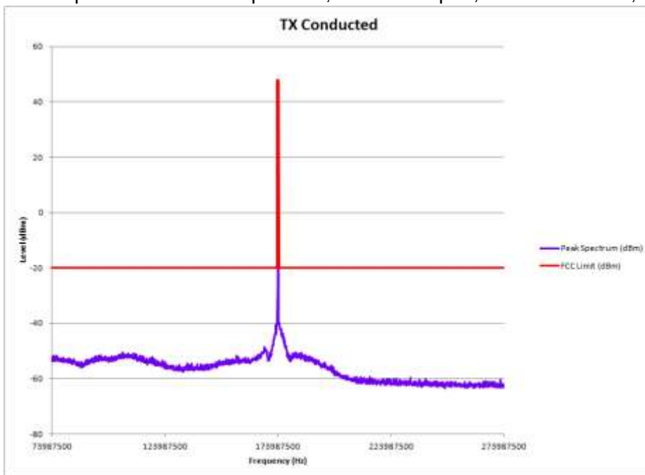
E1-6.6 Conducted Spurious Emission Spectrum, 200 MHz Span, Power 60 Watts, 173.9875MHz
