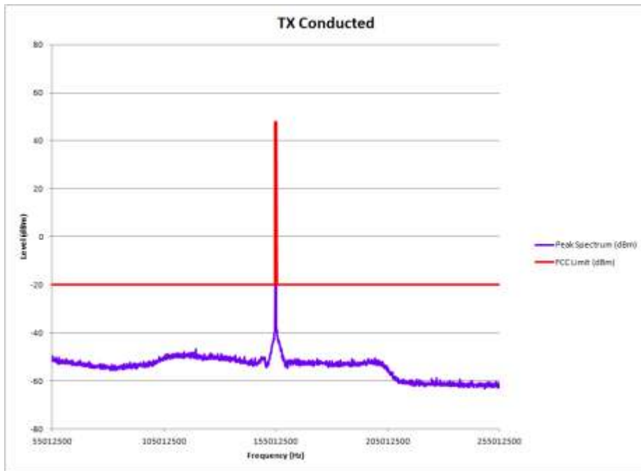
E1-6.5 Conducted Spurious Emission Spectrum, 200 MHz Span, Power 60 Watts, 155.0125MHz
