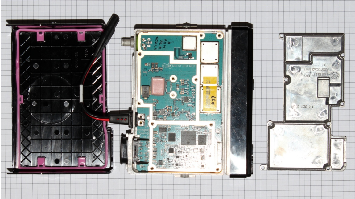
TOP VIEW WITH DECORATIVE COVER AND CHASSIS TOP COVER REMOVED (MATING SURFACES OF TOP COVER AND CIRCUIT BOARD IN CHASSIS ARE SHOWN)
