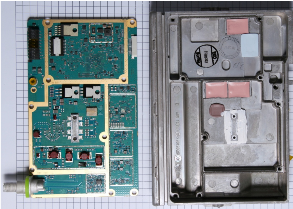
TOP VIEW WITH CIRCUIT BOARD REMOVED FROM CHASSIS AND INDIVIDUAL SHIELDS REMOVED (MATING SURFACES OF CIRCUIT BOARD AND CHASSIS ARE SHOWN)
