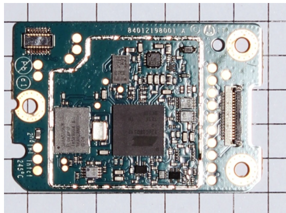
BACK VIEW OF OPTION BOARD WITH INDIVIDUAL SHIELD REMOVED
