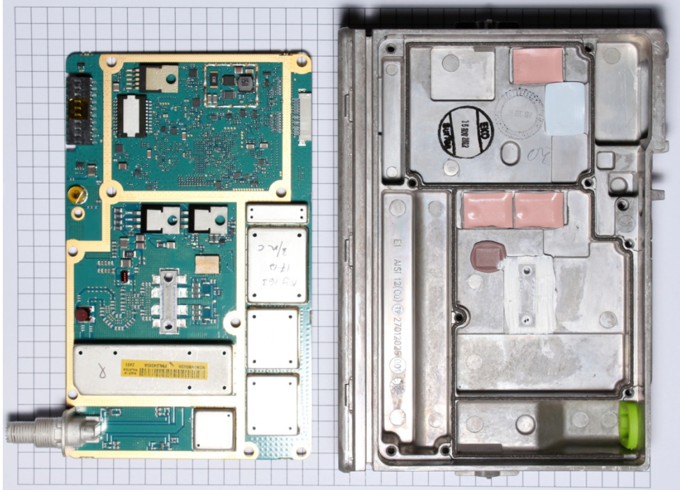
TOP VIEW WITH CIRCUIT BOARD REMOVED FROM CHASSIS (MATING SURFACES OF CIRCUIT BOARD AND CHASSIS ARE SHOWN)
