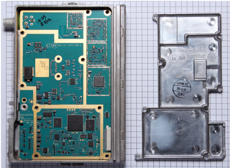
TOP VIEW WITH CHASSIS TOP COVER REMOVED AND INDIVIDUAL SHIELDS REMOVED (MATING SURFACES OF TOP COVER AND CIRCUIT BOARD IN CHASSIS ARE SHOWN)
