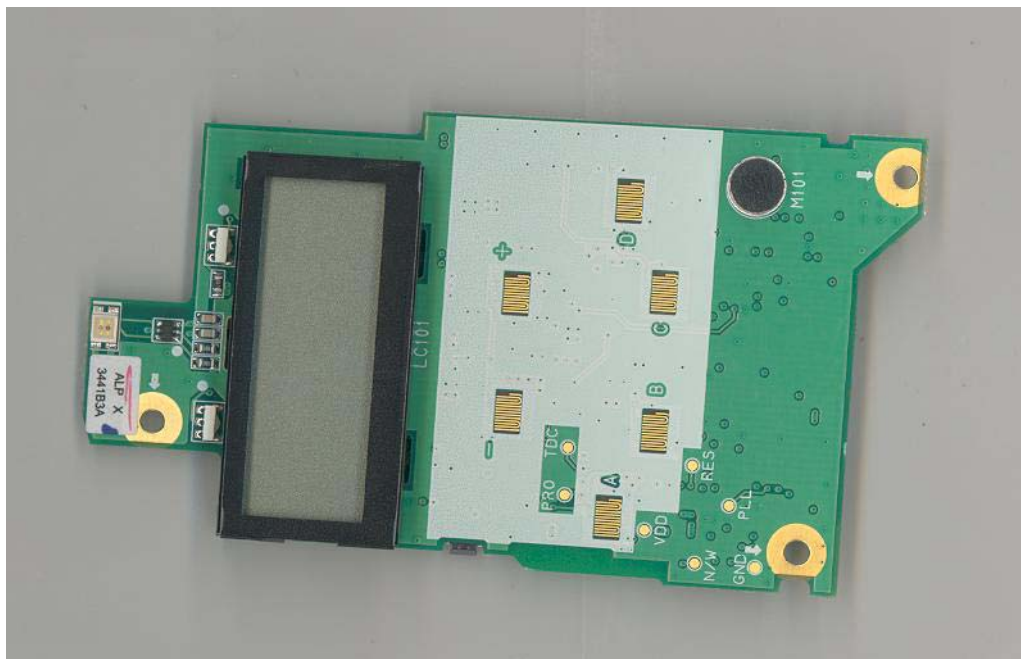
Figure 9-3: Top Side of Controller PCB.
