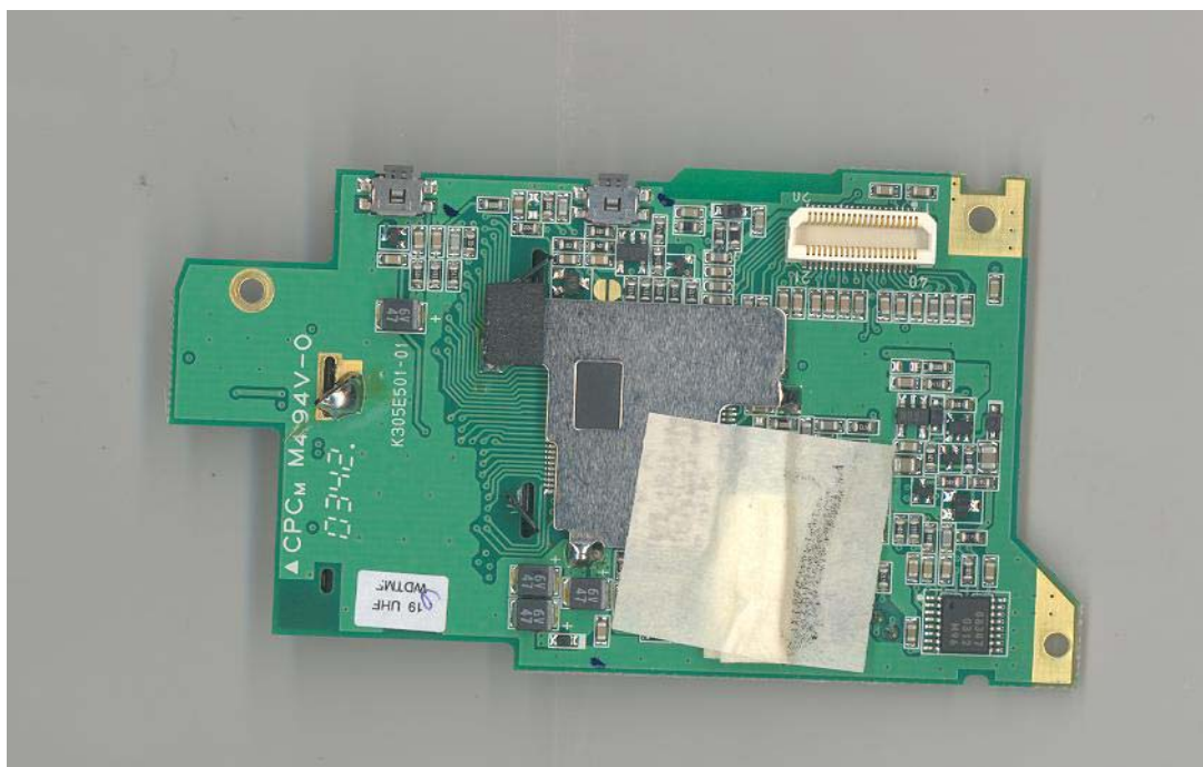
Figure 9-4: Bottom Side of Controller PCB with shields.
