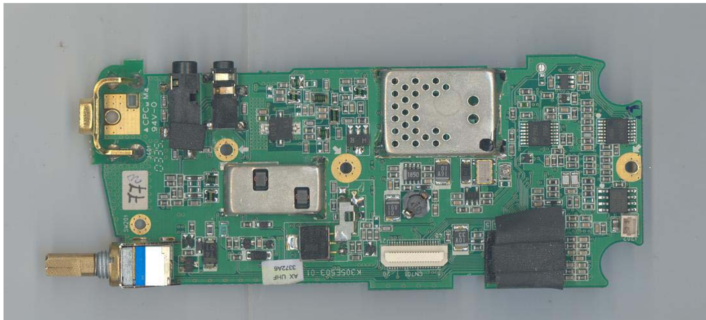
Figure 9-1: Top Side of RF PCB.
