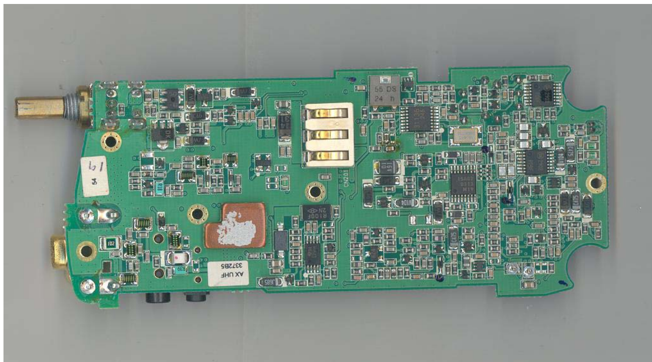
Figure 9-2: Bottom Side of RF PCB.
