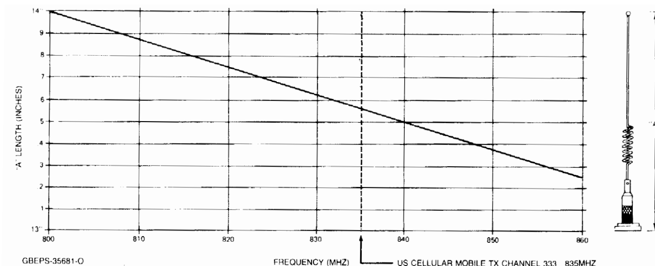
Figure 14. Antenna Tuning Chart
