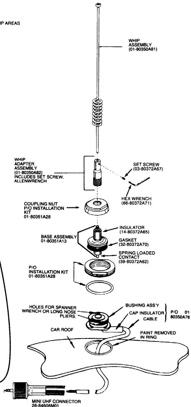
Figure 11. Model shown is a complete antenna RRA-4914
