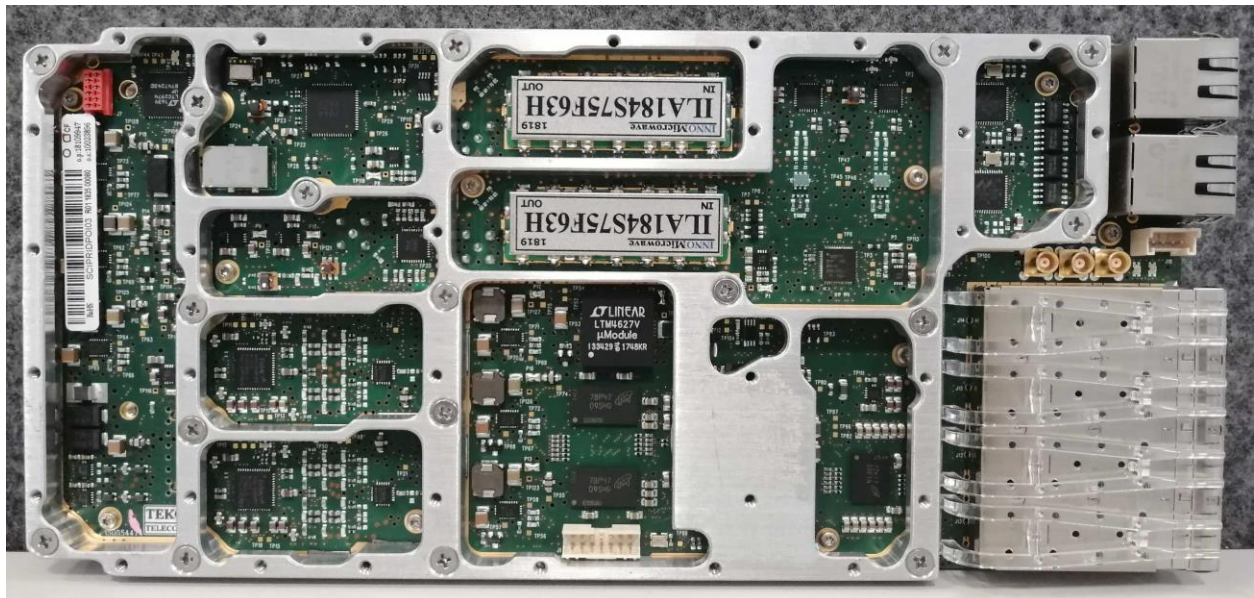
Digital Board final assembly (with grid)
