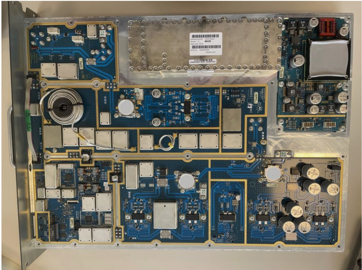
D3-5 Internal Top View - Power Amplifier Module
