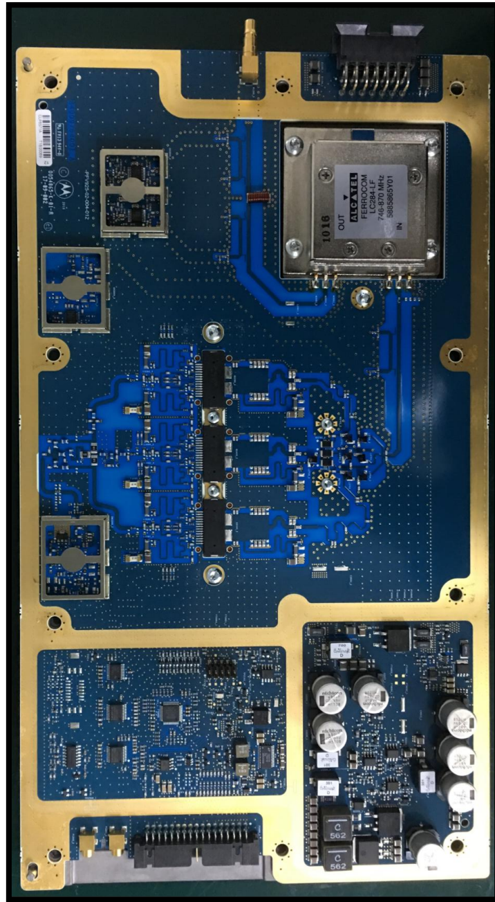
Power Amplifier Circuit Board, Top View for MTS 2 and MTS 4
