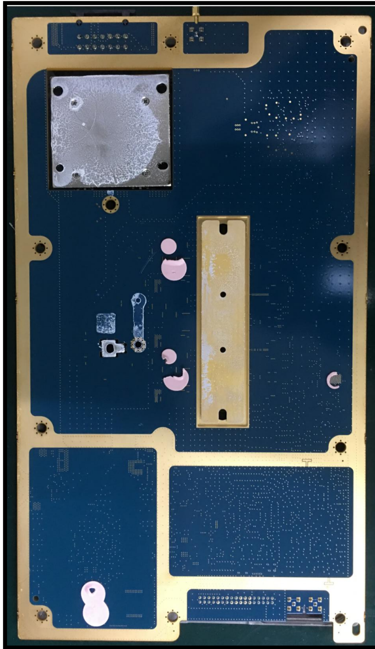
Power Amplifier Circuit Board, Bottom View for MTS 2 and MTS 4
