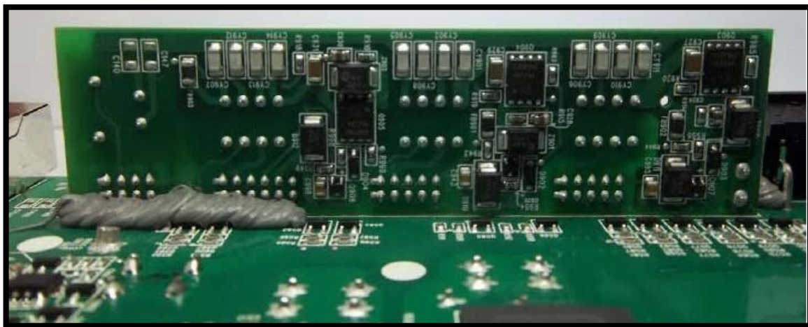
Power Supply Fan Output Board, Front and Back View for MTS 2 and MTS 4
