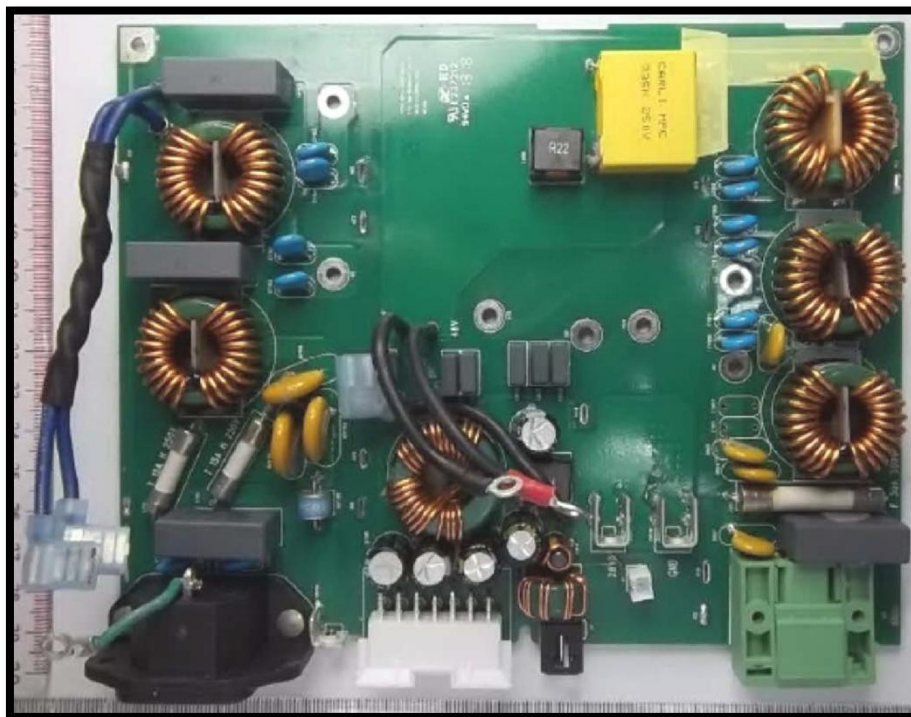
Power Supply Input Connector with and without Shields, Top View for MTS 2 and MTS 4
