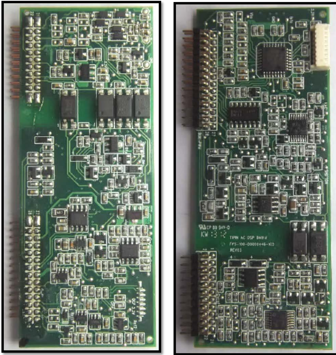
Power Supply AC DISP Board, Top and Bottom Side for MTS 2 and MTS 4
