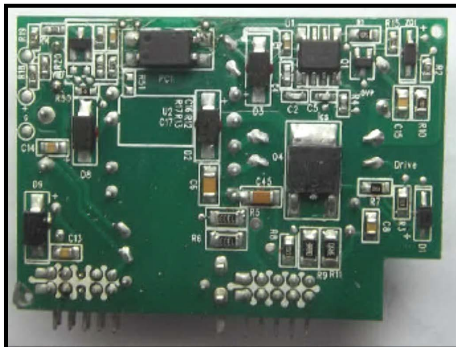
Power Supply AC Aux Board, Top and Bottom Side for MTS 2 and MTS 4
