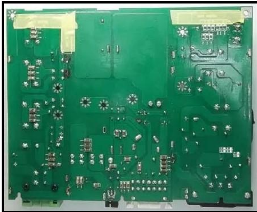
Power Supply Input Connector with and without Shields, Bottom Side for MTS 2 and MTS 4
