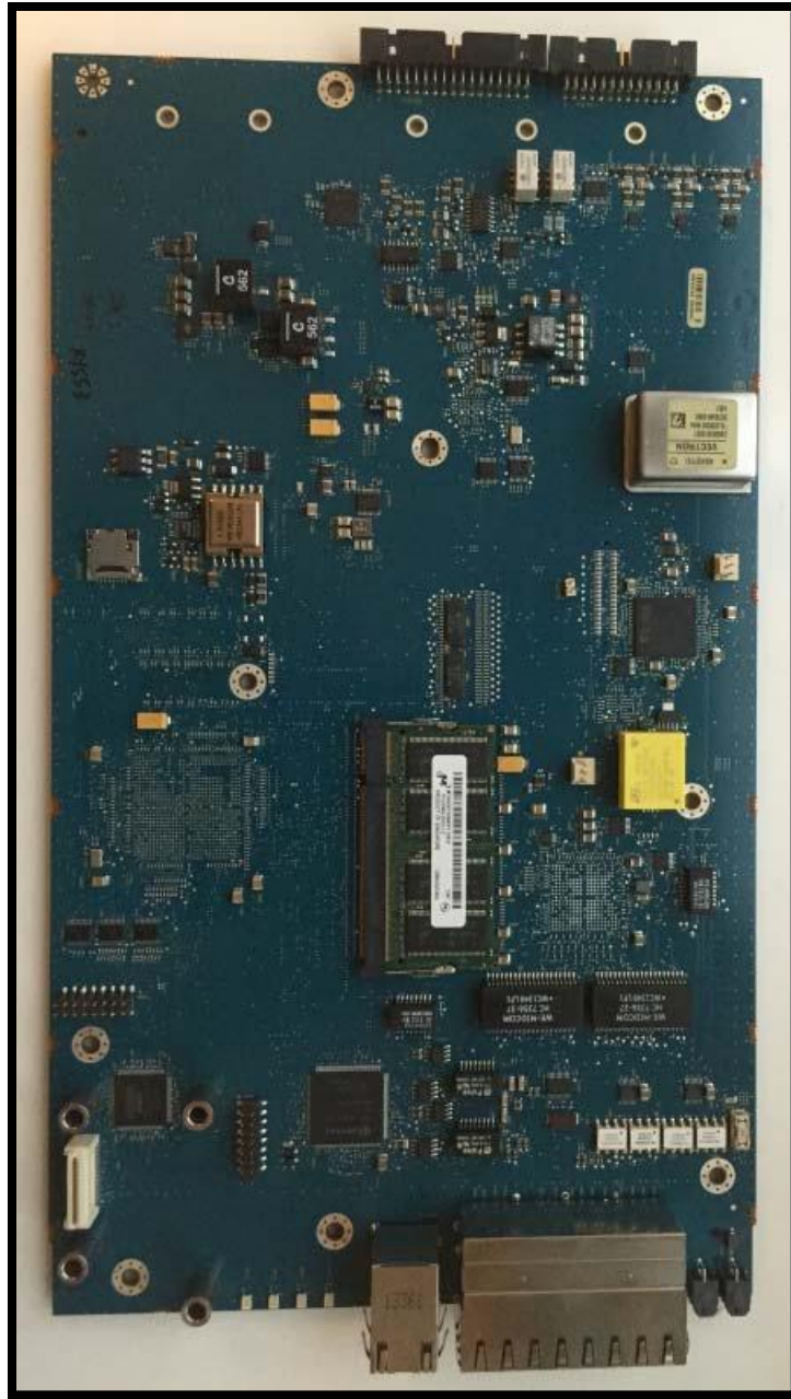
Site Controller Circuit Board, Top View for MTS 2 and MTS 4
