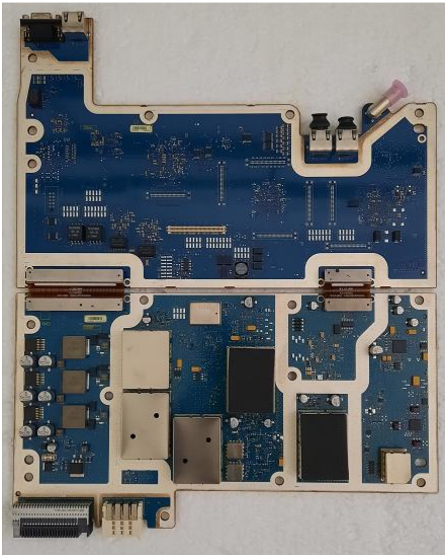
Exhibit 9C – Internal Top View – Transceiver Module, Circuit Board
