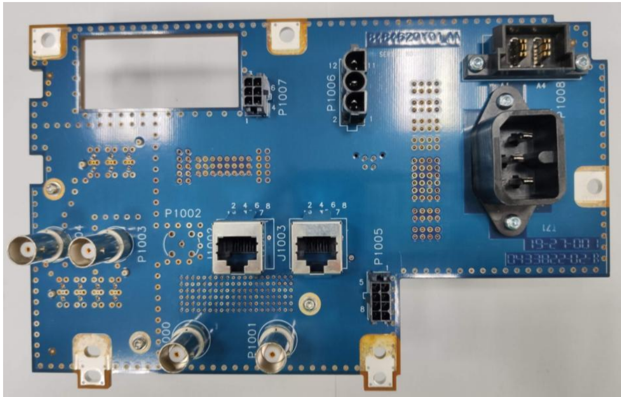
Exhibit 9J – Internal Top View – Backplane
