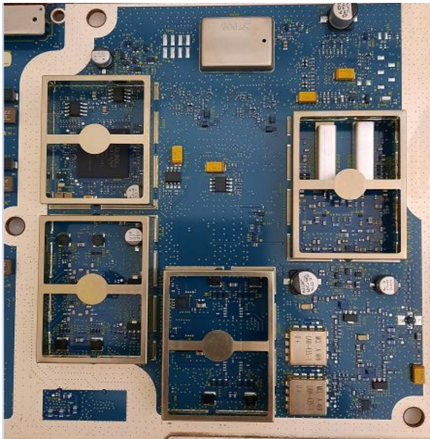
Exhibit 9F – Internal Top View – Transceiver Module, Receiver Section
