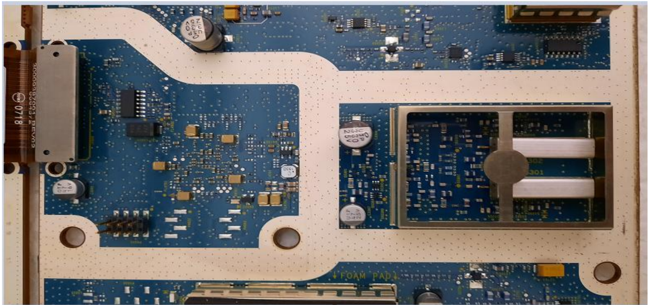
Exhibit 9E – Internal Top View – Transceiver Module, Exciter Section
