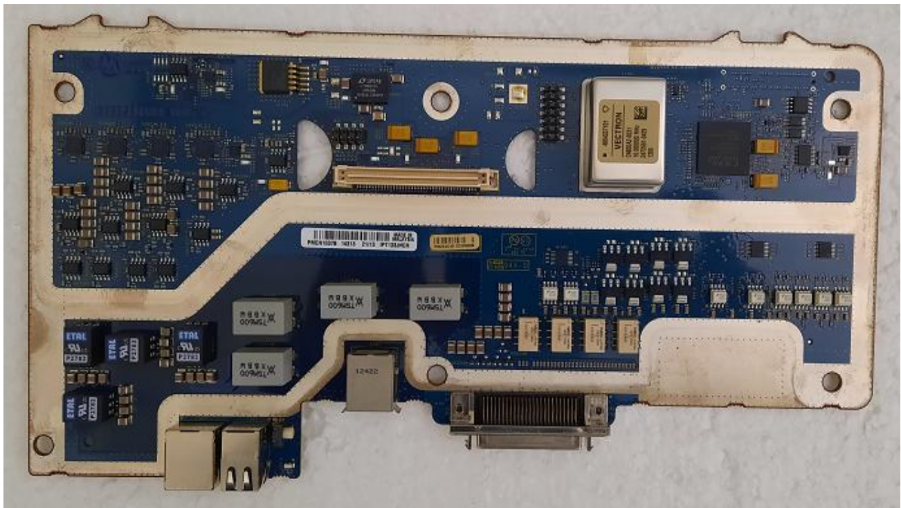
Exhibit 9K – Internal Top View – Transceiver Option Card (TOC)
