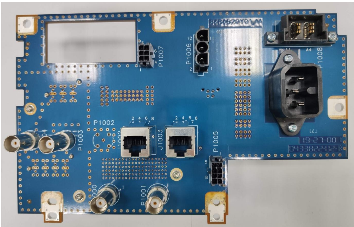
Exhibit 3I – Internal Front View – Backplane
