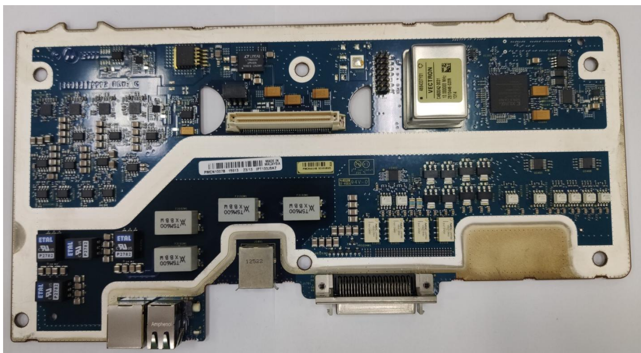
Exhibit 3J – Internal Front View – Transceiver Option Card (TOC)
