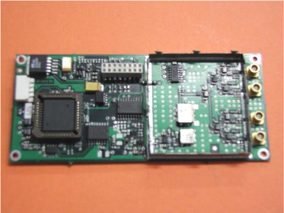
Photo: VSWR Board
