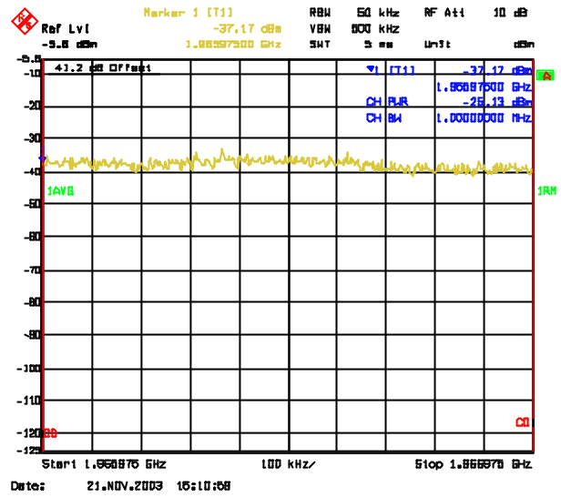
1965.975 MHz-1966.975 MHz
