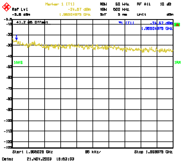
1965.025 MHz-1965.975 MHz
