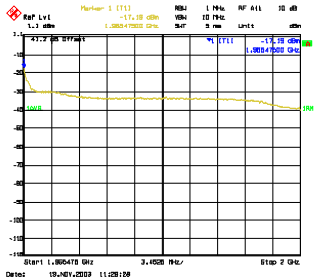
1965.475 MHz-2000 MHz
