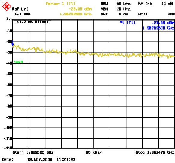
1962.525 MHz-1963.475 MHz
