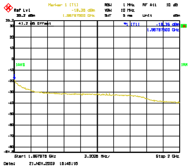
1967.975 MHz-2000 MHz
