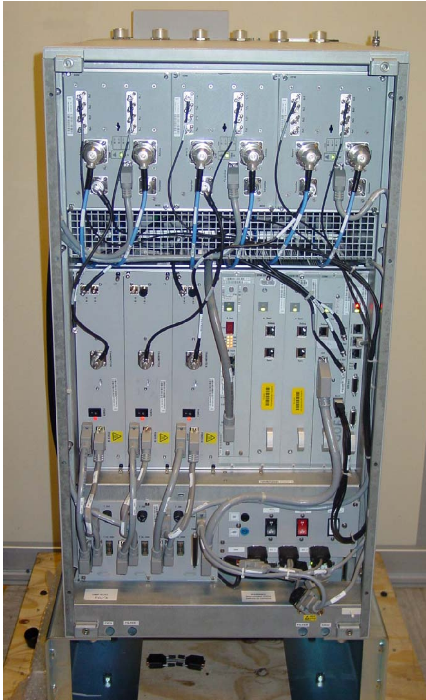
Figure 1: Front view, door removed
