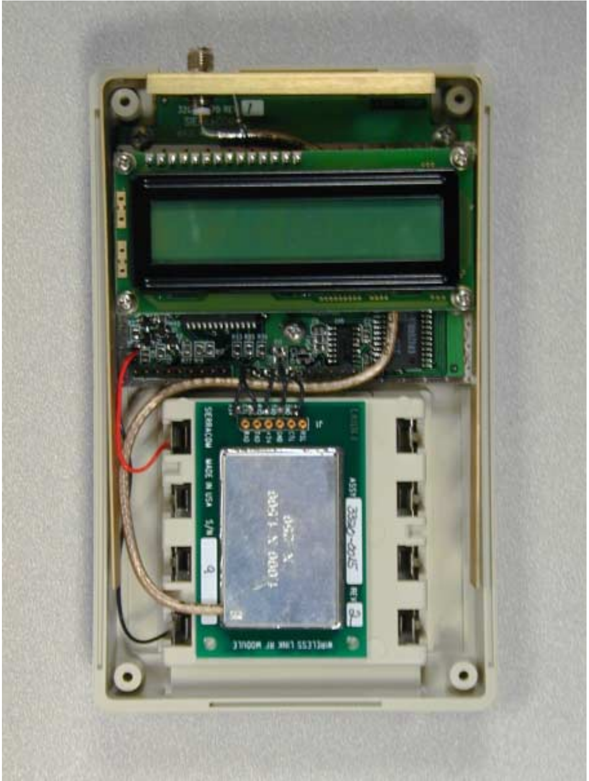
Internal Photos Nortel AB6NTHV45AA
