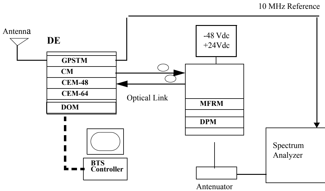
Figure 4 : Test Setup for Spurious Emissions Measurement
