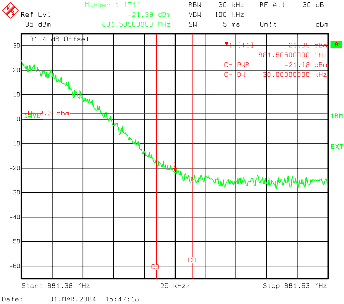
Figure 78 : One Carrier - Industry Canada Upper 750 kHz offset 30 kHz Chan Power Ch 358
