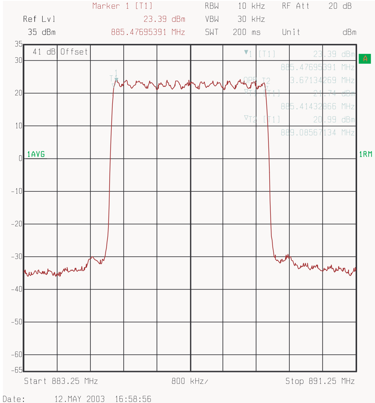
Figure 5 : Occupied Bandwidth - 3 Carrier, Channel 534, 575, 616
