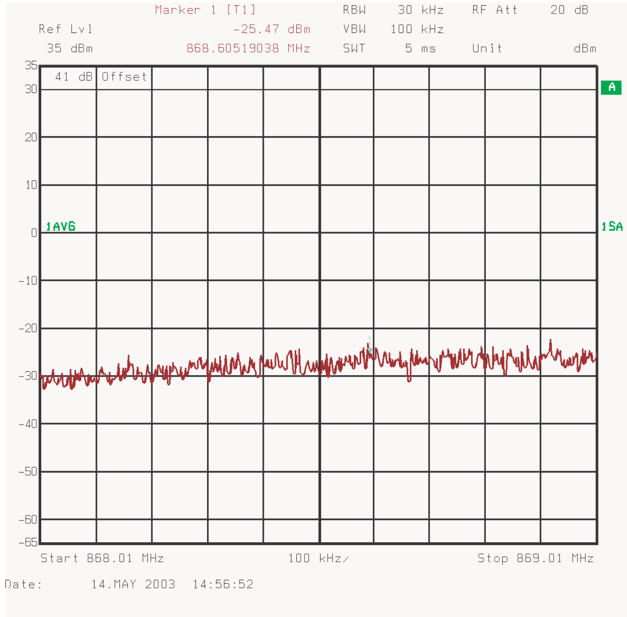
Figure 7 : Conducted Spurious Emissions - 1 Carrier, Channel 17 (Lower adjacent 1 MHz)
