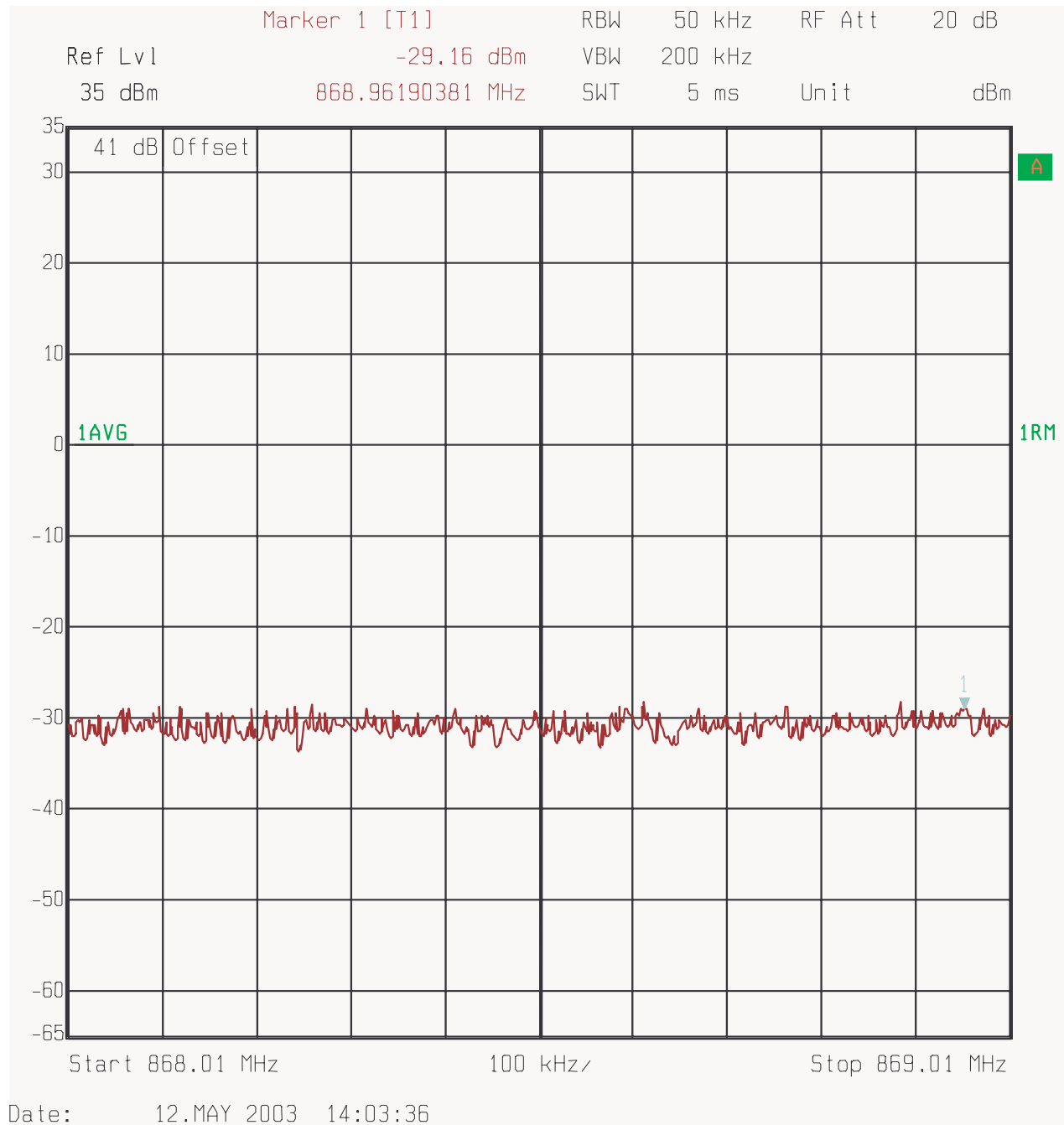
Figure 18 : Conducted Spurious Emissions - 3 Carrier, Channels 17, 58, 99 (Lower adjacent 1 MHz)
