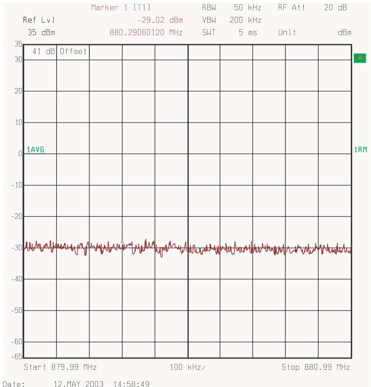
Figure 19 : Conducted Spurious Emissions - 3 Carrier, Channels 201, 242, 283 (Upper adjacent 1 MHz)
