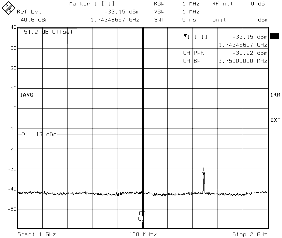
Figure 25 : Conducted Spurious Emissions - 3 Carrier, Channels 8, 49, 90 (1 GHz - 2 GHz)
