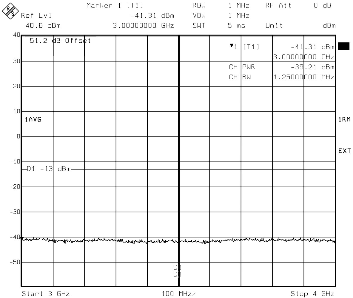
Figure 15 : Conducted Spurious Emissions - 1 Carrier, Channel 8 (3 GHz - 4 GHz)
