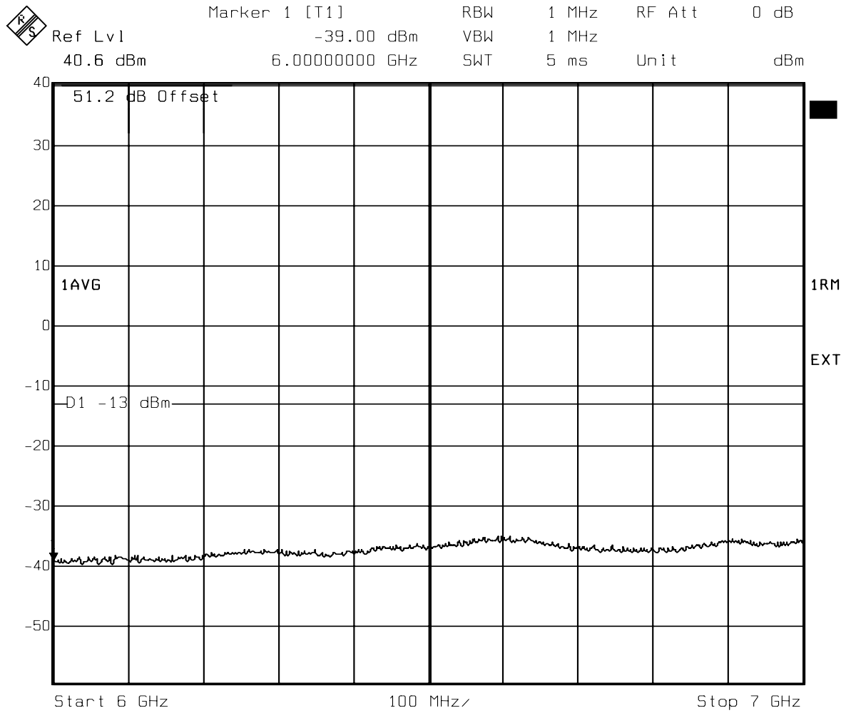
Figure 18 : Conducted Spurious Emissions - 1 Carrier, Channel 8 (6 GHz - 7 GHz)
