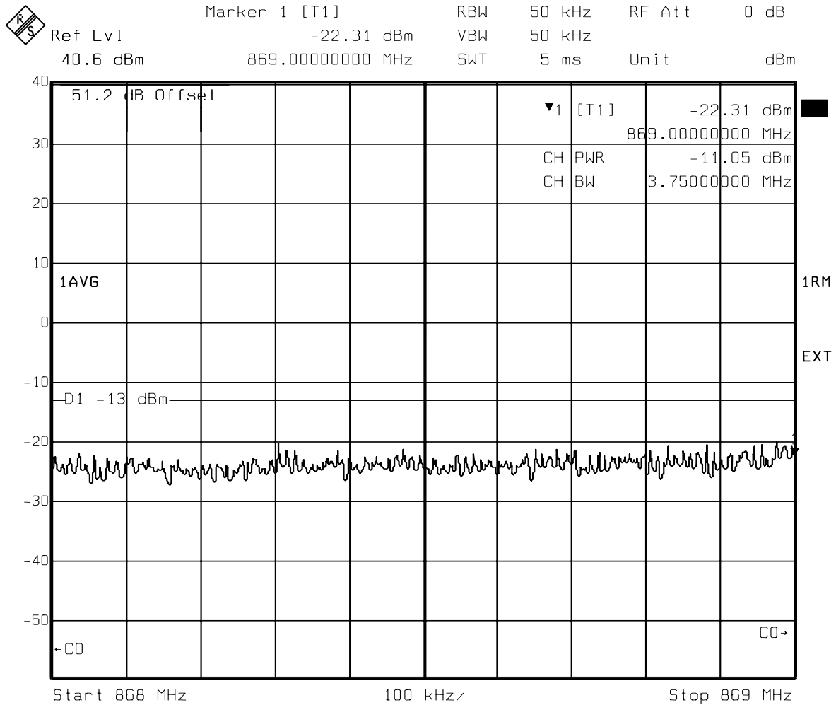
Figure 21 : Conducted Spurious Emissions - 3 Carrier, Channels 8, 49, 90 (Lower adjacent 1 MHz)
