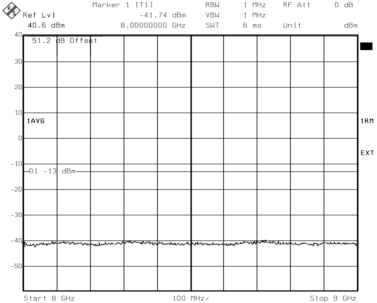
Figure 20 : Conducted Spurious Emissions - 1 Carrier, Channel 8 (8 GHz - 9GHz)
