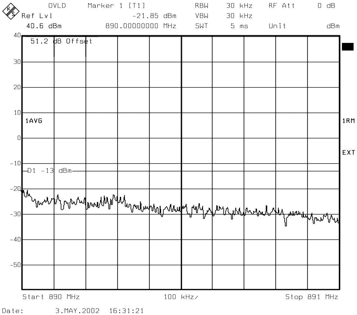
Figure 8 : Conducted Spurious Emissions - 1 Carrier, Channel 616 (Upper adjacent 1 MHz)
