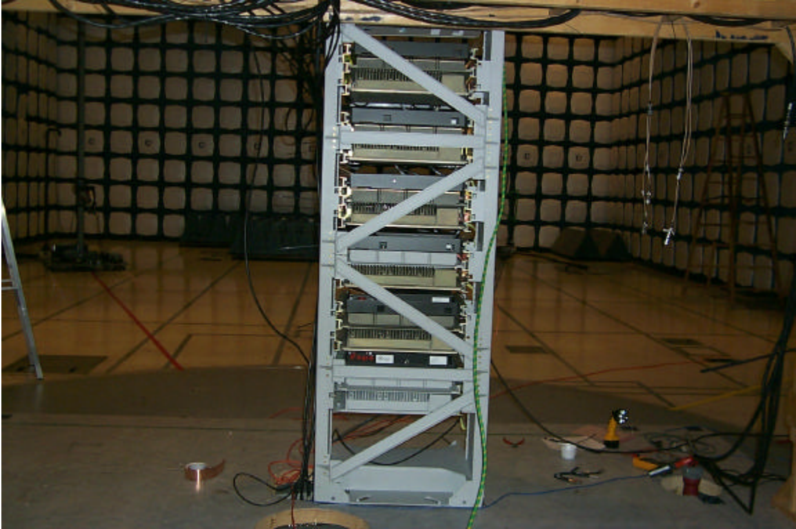
Test Set-up Picture 3: 6 MFRM Radio (Back View)
