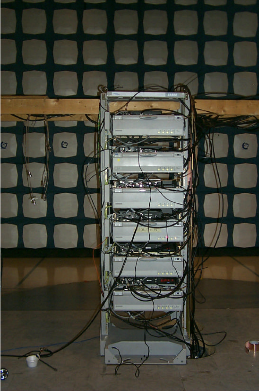
Test Set-up Picture 1: 6 MFRM Radios (Front View)
