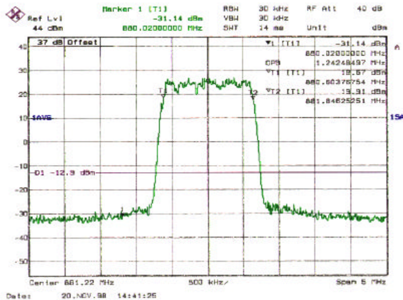
Figure 7: Spurious Emissions (Channel 374)
